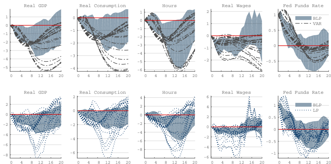
FIGURE 5: STABILITY OVER SUBSAMPLES: VAR, LP AND BLP
