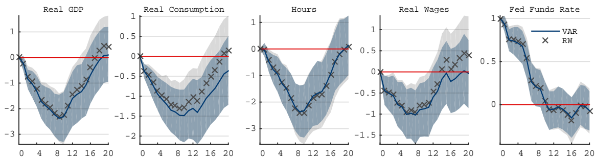
FIGURE 2: BLP RESPONSES: VAR VS RW PRIOR
