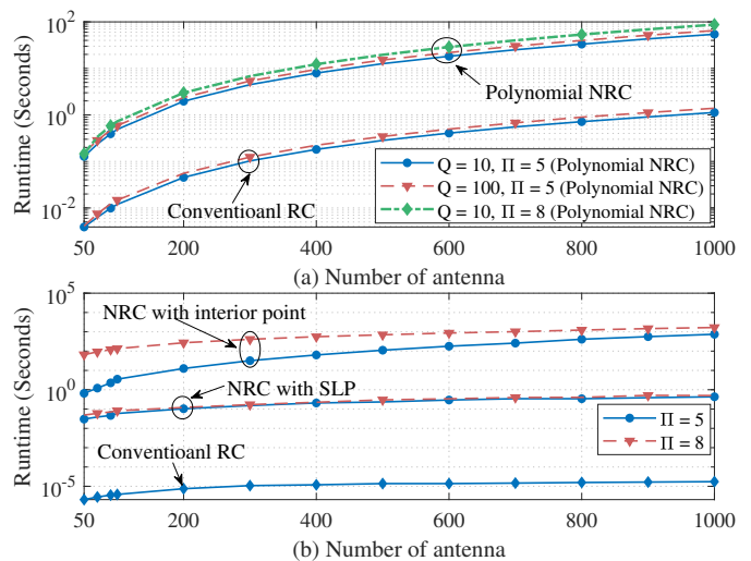
Fig. 10. Complexity of the conventional NRC and the polynomial NRC versus the antenna number.
