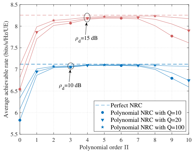
Fig. 8. Average achievable rate after RC versus the polynomial order \Pi .
