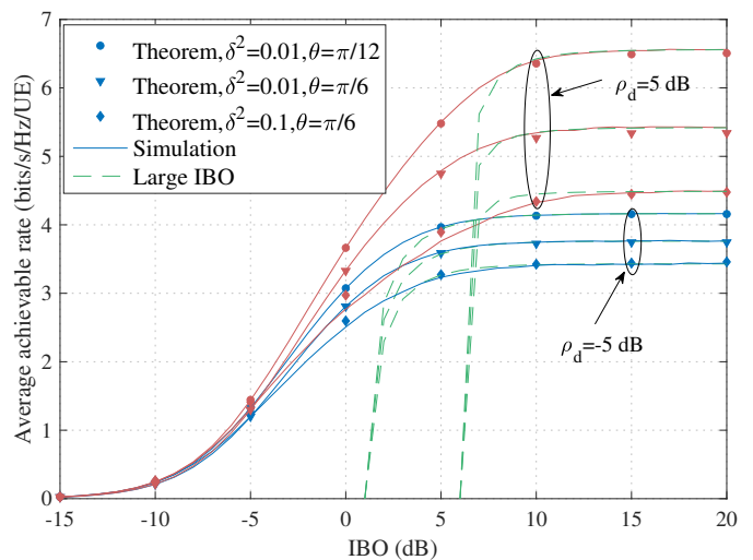
Fig. 5. Average achievable rate versus IBO.
