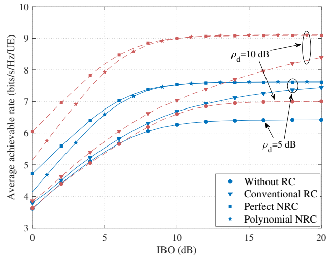
Fig. 7. Average achievable rate after the RC versus IBO.
