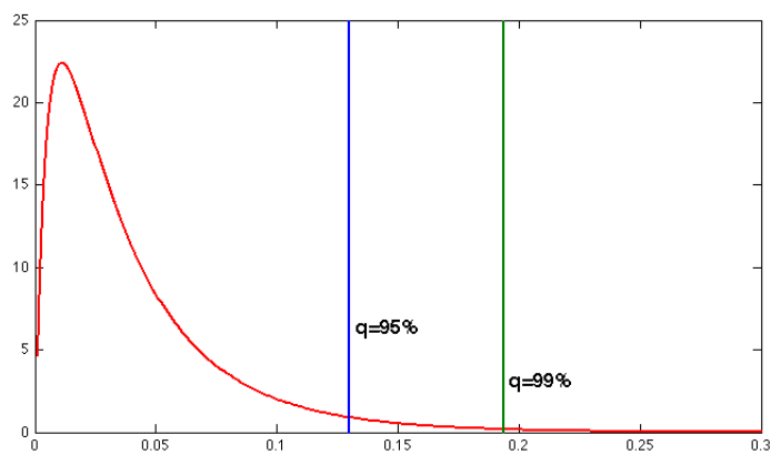
Figure 2.8: PD = 5\% , \rho = 13\%
