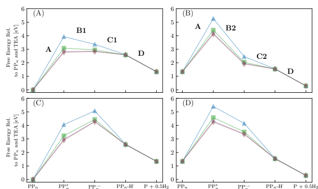
Fig. 8 The predicted free energy profile for each step in H 2 O of sub-cycle I (A) and II (B). The predicted free energy profile for each step in TEA of sub-cycle I (C) and II (D). Data shown for n = 2 (blue triangles), 4 (green squares), 6 (purple stars) and 7 (brown diamonds), calculated using B3LYP and provided relative to PP n and TEA. For the equivalent data calculated with CAM-B3LYP see Fig. S3.
