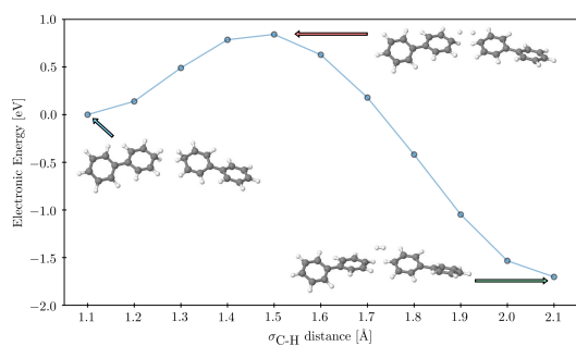
Fig. 7 Predicted energy profile for the H 2 formation step showing the energy of each geometry along the constrained optimization scan. All values calculated with B3LYP/cc-pVTZ for PP 2 -H 2 O.
