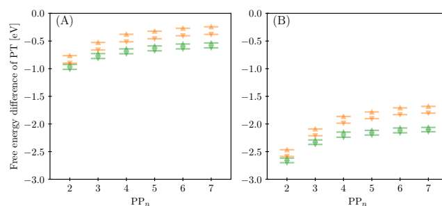
Fig. 6 Predicted free energy difference of proton transfer to the oligomer at the C_3 position as a function of oligomer length for PP_n - H_2O (A) and PP_n -TEA (B), when TEA^{*\bullet} (upward triangle) and TEAR^+ (downward triangle) are the source of protons. B3LYP results in orange and CAM-B3LYP results in green.
