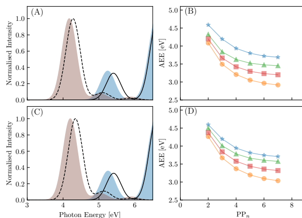
Fig. 4 The simulated absorption spectra for PP 2 (blue) and PP 7 (brown) in H 2 O calculated using TD-CAM-B3LYP (A) and the predicted AEE as a function of oligomer length for CAM-B3LYP (green triangles), SCS-ADC(2) (blue stars), B3LYP (orange circles) and MN15 (red squares) for PP n oligomers in H 2 O (B). The simulated absorption spectra for PP 2 (blue) and PP 7 (brown) in TEA calculated using TD-CAM-B3LYP (C) and the predicted AEE as a function of oligomer length for CAM-B3LYP (green triangles), SCS-ADC(2) (blue stars), B3LYP (orange circles) and MN15 (red squares) for PP n oligomers in TEA (D). In A and C the SCS-ADC(2) equivalent is given as a solid or dashed black line for PP 2 and PP 7 , respectively.
