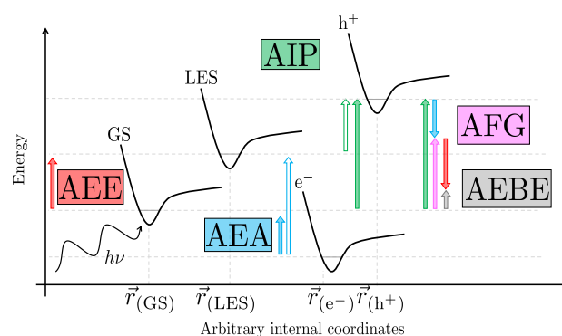
Fig. 3 Schematic illustration of various energetic terms of interest: adiabatic excitation energy (red arrow), adiabatic electron affinity (blue arrow), adiabatic ionization potential (green arrow), adiabatic fundamental gap (pink arrow) and the adiabatic exciton binding energy (grey arrow), while the excited state adiabatic electron affinity and ionization potential are also illustrated (hollow blue and green arrow, respectively). As we consider adiabatic values in all cases we use energies based on the equilibrium arrangement for each electronic configuration, this has been represented by a general potential energy surface (black curve) for the ground (GS), lowest excited (LES), one-electron reduced ( e^- ) and one-electron oxidized state ( h^+ ), with the location of the minimum energy arrangement varying for each.
