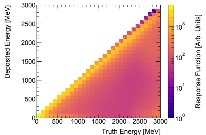
FIG. 27. The average calorimeter response function showing the deposited energy vs. the truth energy, integrated over the decay volume.
