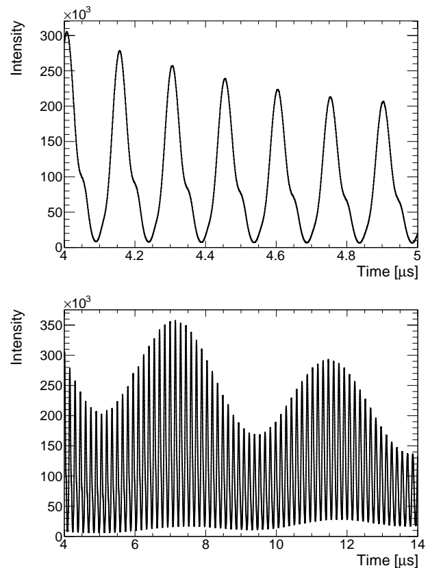
FIG. 4. Positron counts as a function of time as seen by all the calorimeters combined for the Run-1d data set for the time ranges: (top) 4–5 \mu\text{s} and (bottom) 4–14 \mu\text{s} with respect to the beam injection. The time binning period is 1 ns. The amplitude modulation in the bottom panel is from the muon spin rotation frequency \omega_a^m .
