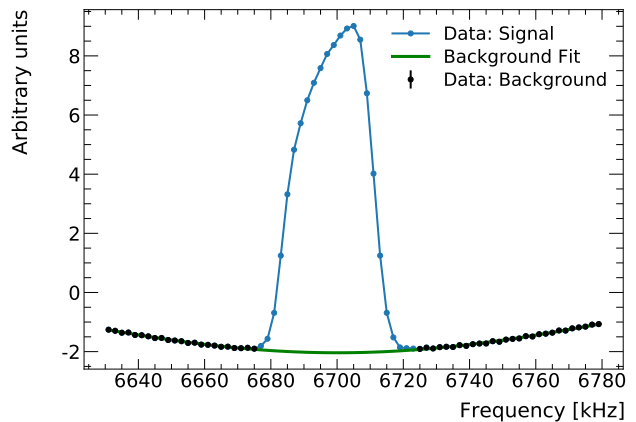
FIG. 5. The frequency distribution obtained with a cosine transform of the fast rotation signal from the Run-1d data set. The background is a consequence of the missing data before the start time of 4 \mu\text{s} . A cardinal sine (sinc) background fit has been applied to the black points and is subtracted from the whole frequency range as a correction.
