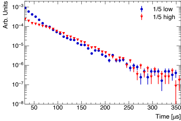
FIG. 17. The muon loss function L(t) , normalized to beam intensity, for the lowest (blue) and highest (red) momentum stored momentum distributions; see corresponding momentum distributions in Fig. 16. Asymmetry in the loss rates is seen early in the fill.
