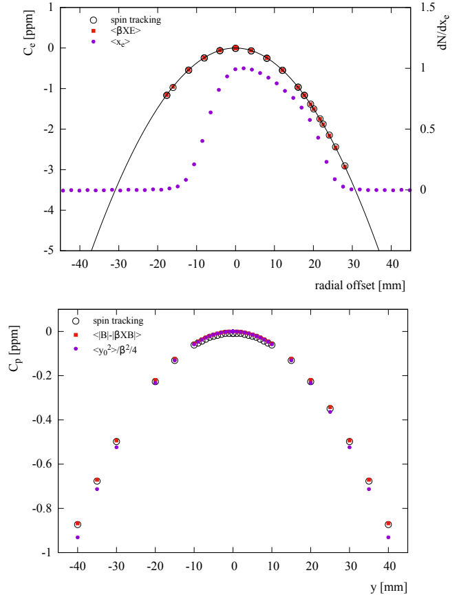
FIG. 25. Top: Contribution to \omega_a due to the electric field as computed by spin tracking (integration of the Thomas-BMT equation) and integration along trajectories (Eq. B3) for closed orbits at varying radial offsets. The vertical closed orbit is zero and there is no vertical betatron motion. A representative, measured radial distribution is superimposed for reference. Bottom: Contribution to \omega_a due to the vertical oscillation computed with spin tracking and integration along the trajectory (Eq. B4) for muons with magic momentum and zero radial betatron amplitude. Note that the formula that assumes linearity overestimates the contribution at large amplitudes.
