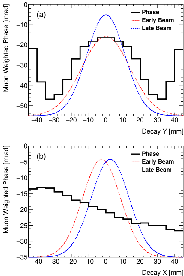
FIG. 21. Phase vs. vertical (a) and horizontal (b) decay coordinate. The Gaussian profiles show (at an exaggerated scale) how muon distributions might evolve from early (dotted red) to late (dashed blue) times in the fill. The largest effect is from the reduction in the vertical width (a), where the phase changes to the distribution add coherently. The mean shift (not shown) is smaller because the increase on one side is balanced on the opposite side. Conversely, the larger phase shift in the radial projection is from the mean motion (b), while the width change (not shown) is largely cancelled.
