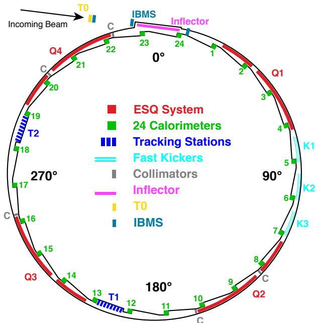
FIG. 2. Plan view of the g-2 storage ring vacuum chamber and instrumentation highlighting the important components discussed in this paper. The beam enters through a field-free corridor provided by the inflector magnet. Three kicker stations operate in concert to deflect the beam onto a stable orbit during the first turn. Four quadrupole stations, each consisting of a short and long section, provide vertical containment. The T0 and IBMS detectors monitor the injected beam intensity, time profile, and spatial distribution.
