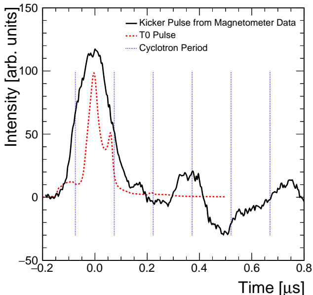
FIG. 1. The solid black trace represents the shape of the kicker magnetic field. The ringing is owing to an unavoidable impedance mismatch. The dashed red trace represents the average injected muon bunch temporal intensity distribution as measured by the T0 detector. The vertical dotted lines are separated by the 149 ns cyclotron period. The overlay between kicker and beam shapes shows that not all entering muons experience the same magnetic deflection. It is clear from the ringing that muons experience multiple kicks, both inward and outward.
