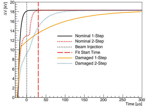
FIG. 3. Charging profiles for the 30 nominal quadrupole plates driven by either 1-step (black) or 2-step (dotted red) power supplies. The two damaged resistors (solid orange and dotted blue), connected to the same 1- and 2-step power supplies, exhibit markedly different charging profiles during the data fitting period. The vertical dotted black line at time t = 0 represents the arrival time of the muons in the storage ring. The vertical dashed red line at 30 \mu\text{s} indicates the time at which the precession data fits begin. The resistors deteriorated slightly for Run-1d and the precession fit start time was delayed to 50 \mu\text{s} to compensate for the longer time charging profiles.
