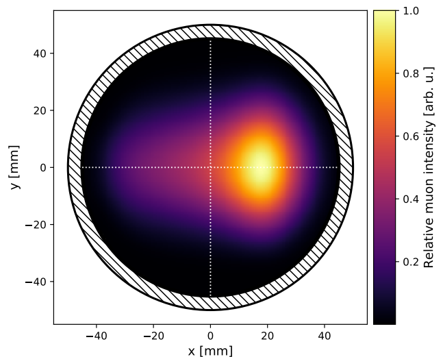
FIG. 19. An azimuthally-averaged muon spatial distribution for Run-1a as measured by the trackers. The (hatched) collimator defines the 45-mm-radius transverse storage aperture.
