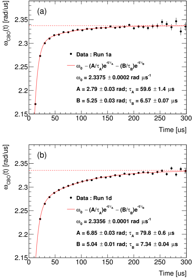
FIG. 10. Tracker measurements of \omega_{\text{CBO}} in different time slices during the muon fill from the 270^\circ tracker station. (a) and (b) show the Run-1a and Run-1d data sets, respectively. The fit function and parameters are noted in the figure, together with their uncertainties. The difference between the two data sets is attributed to worsening performance of the damaged ESQ resistors. The time-dependence of the frequency is included in the fits of the positron data from the calorimeters to accurately incorporate the CBO acceptance dependence.
