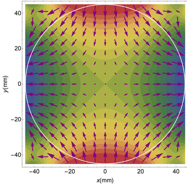
FIG. 23. 2D representation of the equipotentials and electric field in the ESQ region. The circle at radius 45 mm represents the storage ring aperture defined by the collimators.
