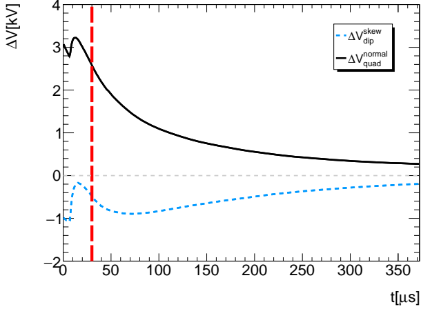
FIG. 8. Additional electrostatic potential at r = 5 cm versus time for the ESQ powered through damaged resistors. The skew dipole (dashed blue) and normal quadrupole (solid black) terms are shown relative to the nominal case and correspond to a 2D Taylor expansion based on data collected after Run-1 using an HV probe. The vertical dashed red line at 30 \mu\text{s} after injection indicates the nominal start of the precession fits. Scraping ends at 7 \mu\text{s} after injection, visible at the abrupt kinks in the curves. Nominal ESQ plates rise with a nominal RC time constant of \tau \approx 5 \mu\text{s} , but these ESQ plates show prolonged and asymmetric time constants which lead to focusing and vertical steering errors during the data taking period.
