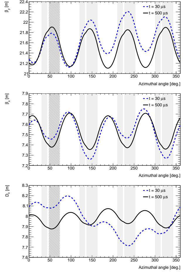
FIG. 9. The calculated \beta_y (top), \beta_x (middle), and dispersion D_x (bottom) functions versus azimuth in the ring at times 30 \mu\text{s} and 500 \mu\text{s} after injection for the Run-1a data set. The calculation includes the effect of the damaged resistors used in the Q1L ESQ section (hatched region) and the measured magnetic field distortions versus azimuth. The vertical shaded regions correspond to the locations in azimuth of the short and long ESQ sections.
