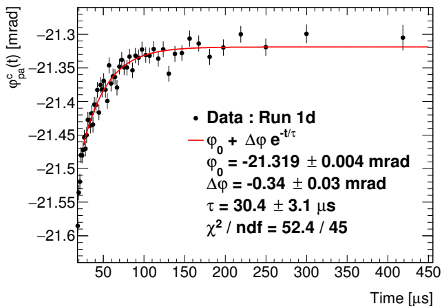
FIG. 22. Calculation of \varphi_{pa}^c(t) for calorimeter 19 in Run-1d using data from the tracker station at 180^\circ and Eq. 26. The fit start time for the extraction of \omega_a^m for this data set is 50 \mu\text{s} after injection in order to mitigate the effect of \varphi_{pa}^c(t) .
