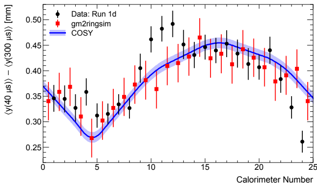
FIG. 12. The change in the vertical mean over the time period from 40 – 300 \mu\text{s} in a fill during Run-1d as measured by the 24 calorimeter stations. The calorimeter data are corrected for acceptance. The blue line corresponds to the COSY model of the vertical closed-orbit evolution during the fill and its prediction of the vertical mean change around the ring. The red squares are from the gm2ringsim muon tracking simulation. This implementation of COSY does not utilize beam tracking so the error band is purely systematic, while the gm2ringsim errors are statistical. Both simulations have been anchored to data from the tracking station at 270^\circ , and have been shifted azimuthally to align with the maximum acceptance for each calorimeter. The azimuthal structure predicted by the simulations due to the damaged resistors is clearly visible in the data.
