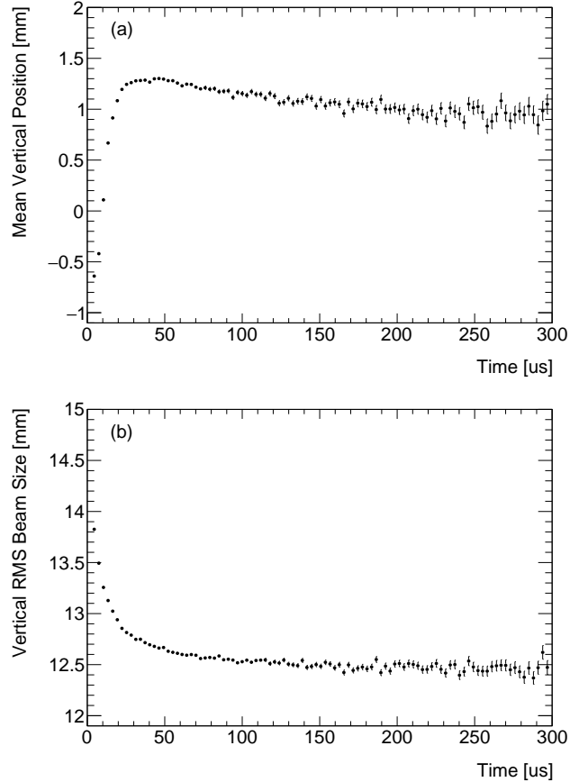
FIG. 11. The 180^\circ tracker station determination of the vertical mean (a) and width (b) versus time-in-fill for Run-1d. The rapid oscillations owing to vertical and horizontal betatron motion have been randomized out to reveal the underlying time-dependence of the mean and width (see also Sec. VIII A).
