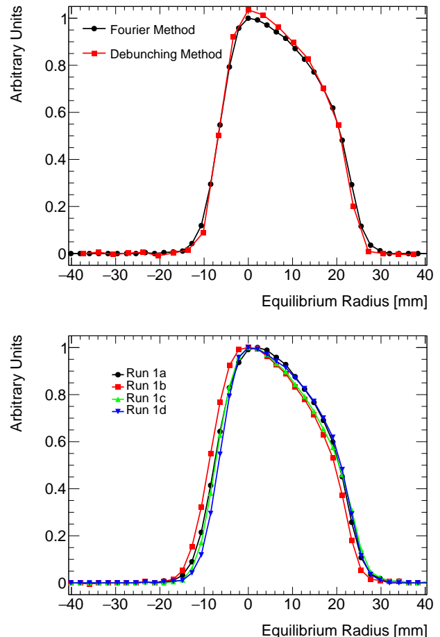
FIG. 6. Top: The radial (closed orbit) distribution extracted by both the Fourier method and the debunching analysis for the Run-1d data set. Bottom: The radial distribution for the four Run-1 data sets as determined by the Fourier method. In both plots, the equilibrium radius is defined such that a magic momentum muon is at 0 mm.
