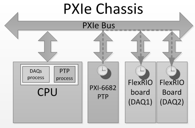
Synchronized DAQ system prototype architecture.
