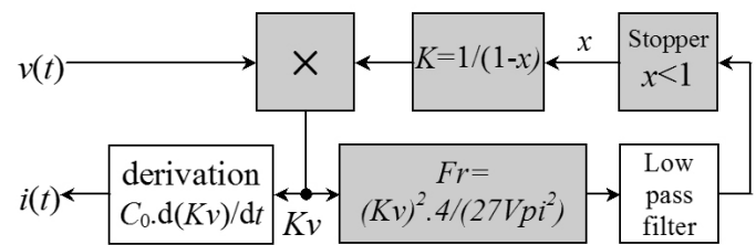
Flowchart of fundamental equations of the MEMS.
