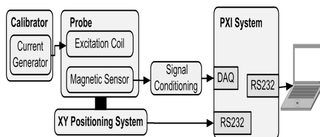
Experimental Setup.
