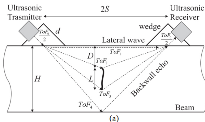
Basic principle of the ToF method
