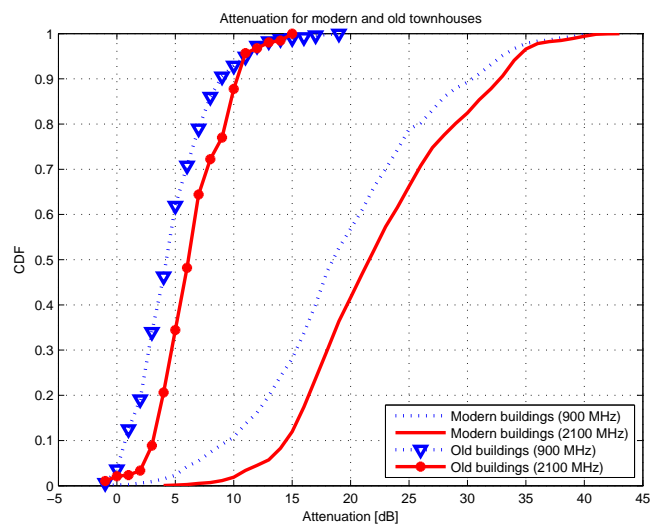
Figure 5. CDF plot for distribution of outdoor-indoor signal level differences for both older and modern townhouses.
