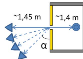
Figure 6. Principal illustration of the experiment setup related to aperture measurements.
