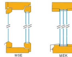
Figure 2. General structures of windows.
