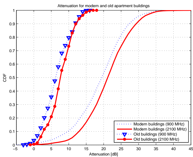
Figure 4. CDF plot for distribution of outdoor-indoor signal level differences for both older and modern apartment buildings.
