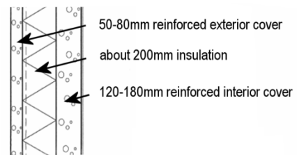
Figure 1. Typical wall sandwich element.
