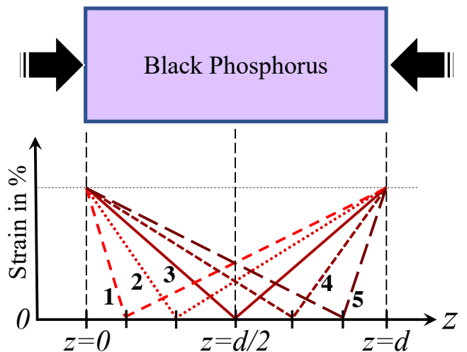
FIG. 6. (Color online). Inhomogeneous strain in the black phosphorous is accounted for by using a linear z -dependent model. The spatially inhomogeneous strain develops along the z direction and it varies linearly (red lines) along the strain direction from a maximum (horizontal dashed line) at locations z = 0 and z = d , to zero strain at points marked by the vertical small indicators at z = d/6, d/3, d/2, 2d/3, 5d/6 . The pertaining curves to these five linear models are marked by 1, 2, 3, 4, 5. The arrows portray the direction of applied strain that propagates linearly inside the BP region confined between z = 0 and z = d .
