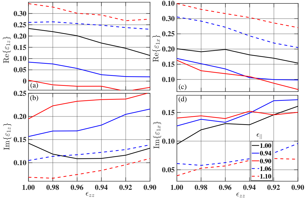
FIG. 7. (Color online). The permittivity of BP as a function of compressive strain \epsilon_{zz} from 0 to -10\% . The panels (a) and (b) show the real and imaginary parts of \epsilon_{1z} whereas the panels (c) and (d) are the real and imaginary part of \epsilon_{1x} . The in-plane strain spans the strain-free, compressive, and tensile strain regimes; \epsilon_{||} = 1.0, 0.94, 0.90, 1.06, 1.10 .
