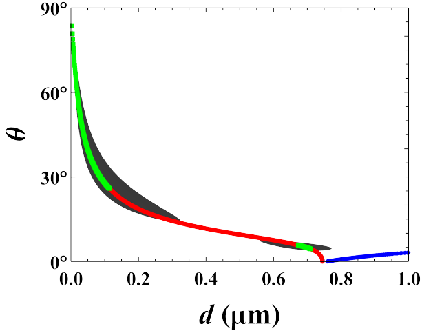
FIG. 9. (Color online). Electromagnetic modes for the system in Fig. 1 with the same parameter values as used in Fig. 5(c). The red curve depicts the fast-wave ( k_{0x}/k_0 < 1 ) waveguide modes, while the green curves correspond to the impedance matched modes (overlapping with the red curve). As the thickness increases, eventually radiative leaky-waves emerge (blue curve). The angle \theta is determined from the propagation constants k_{0x} via \theta = \arcsin(k_{0x}/k_0) . For reference, the black region is extracted from the high absorptance ( > 95\% ) data of Fig. 5(c).
