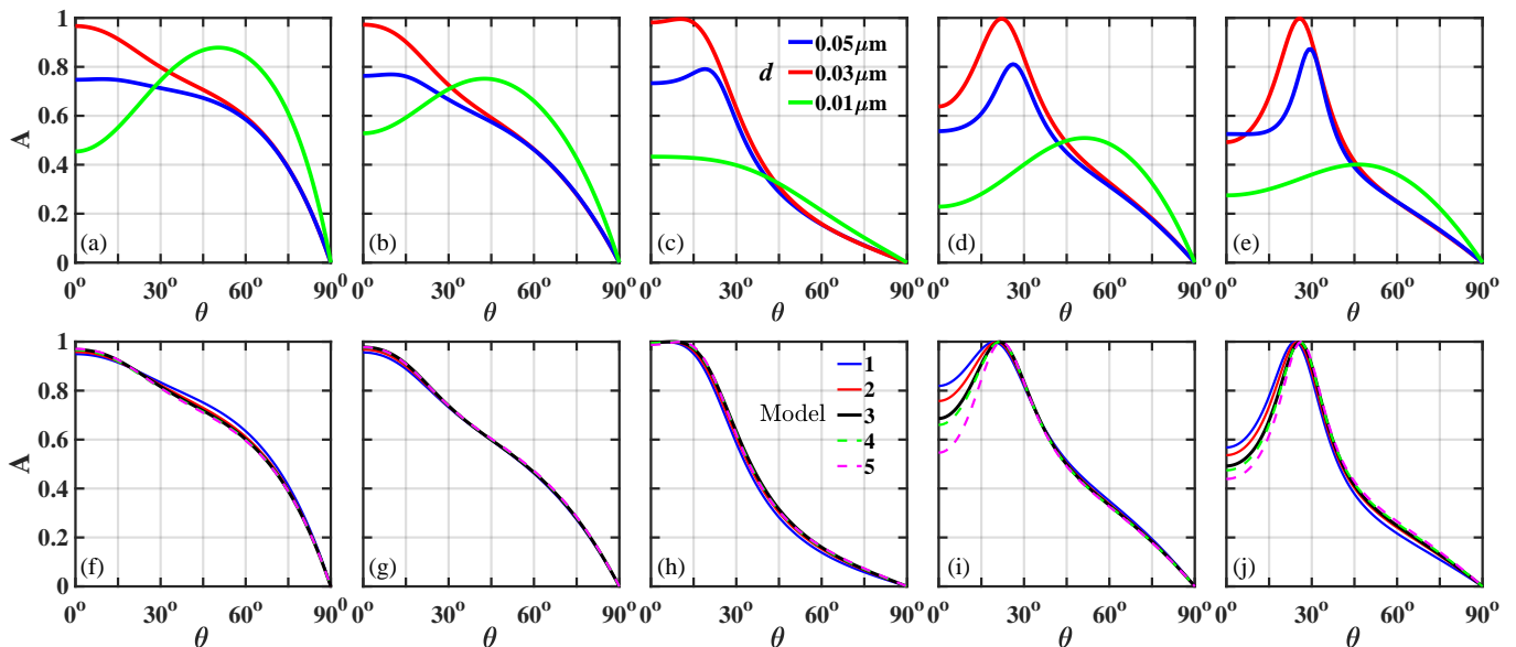
FIG. 8. (Color online). Absorbance vs the incident angle \theta of electromagnetic wave. The frequency of the electromagnetic wave is set to \omega = 22.6 eV. The in-plane strain increases from the leftmost column to the rightmost column, i.e., \epsilon_{\parallel} = -10\% , -6.0\% , 0.0\% , +6.0\% , +10\% in (a,f), (b,g), (c,h), (d,i), and (e,j), respectively. In the top row panels, three different thicknesses of BP are set; d = 0.5\mu\text{m} , 0.3\mu\text{m} , 0.1\mu\text{m} , when model 1 is implemented. In the bottom row panels, the thickness of BP is set to d = 0.3\mu and the five different models (marked by 1, 2, 3, 4, 5) are implemented.
