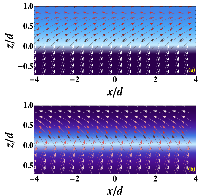
FIG. 3. (Color online). Directional control of energy flow through strain: Two-dimensional maps illustrating the behavior of the time-averaged Poynting vector for a plane wave incident on a black phosphorus film with metallic substrate. The incident angle corresponds to \theta = 34.1^\circ , and the frequency is set at 20.7 eV. In (a) the strain parameters correspond to \epsilon_{\parallel} = 1.04 , leading to perfect absorption, while for (b) the system is unstrained ( \epsilon_{\parallel} = 1 ). For both cases there is no strain in the z direction ( \epsilon_{zz} = 1 ). The film thickness is d = 5.42 \times 10^{-3} \mu\text{m} . The interface separating the black phosphorus from the vacuum region is located at z = 0 and the vacuum region corresponds to z < 0 .
