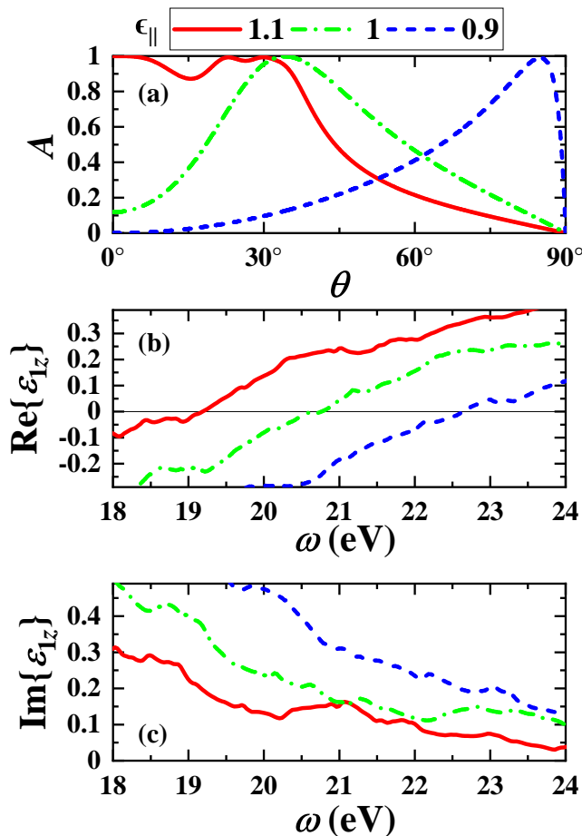
FIG. 4. (Color online). (a) Absorptance as a function of the incident angle \theta for three in-plane strains \epsilon_{\parallel} , as shown in the legend. The frequency is set at \omega = 22.6 eV. (b, c) The corresponding real and imaginary parts of the permittivity component \epsilon_{1z} (obtained by DFT) are shown as a function of the incident wave frequency.
