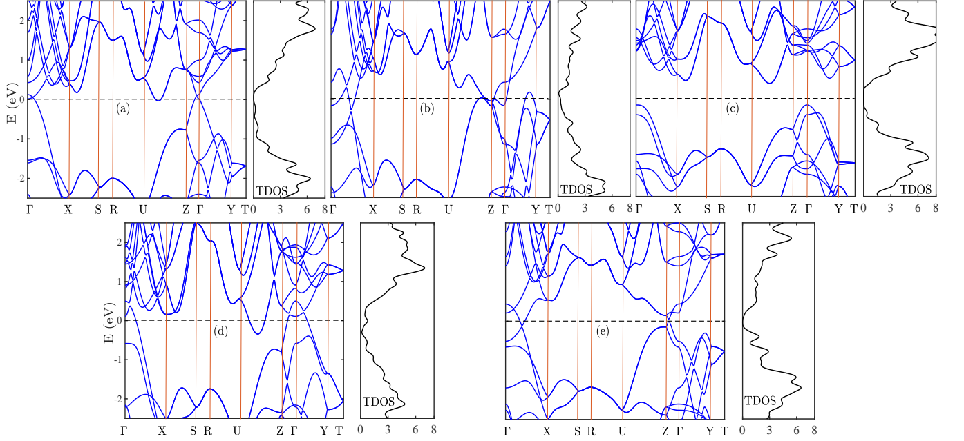
FIG. 10. (Color online). Electronic band structures and total densities of states for bulk black phosphorus. The strain parameters are as follows: (a) \epsilon_{\parallel} = 1.0 , (b) \epsilon_{\parallel} = 0.9 , and (c) \epsilon_{\parallel} = 1.1 for in-plane strain, and (d) \epsilon_{zz} = 0.9 and (e) \epsilon_{zz} = 1.1 for out-of-plane strain. In (a)-(c) the system is unstrained along z ( \epsilon_{zz} = 1 ), and there is no in-plane strain in (d) and (e) ( \epsilon_{\parallel} = 1.0 ). The Fermi energy is located at the energy E = 0 . The axes labels of the top row panels are the same as for the bottom row panels.
