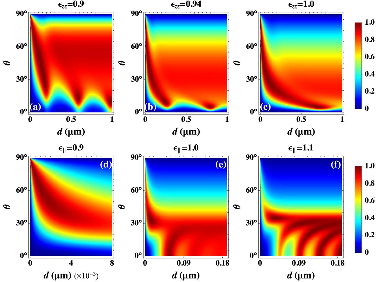
FIG. 5. (Color online). Color maps representing the absorptance as a function of the angle of incidence and thickness of a black phosphorus film with metallic substrate
