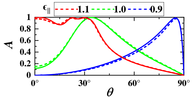
FIG. 12. (Color online). Absorbance ( A ) vs the incident angle \theta for three in-plane strain values \epsilon_{\parallel} = 1.1, 1.0, 0.9 . The frequency of the incident wave is set at \omega = 22.6 eV. The corresponding permittivity components of the dashed and solid lines are obtained using the GLLBsc and PBE functionals, respectively.
