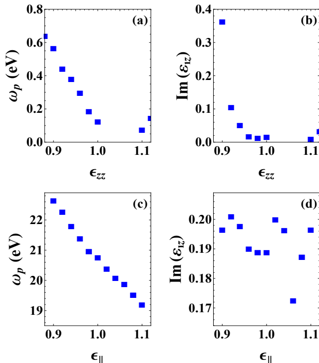
FIG. 2. (Color online). Top row: (a)-(b) Computed frequencies \omega_p from DFT that lead to an ENZ response in bulk black phosphorus as a function of strain \epsilon_{zz} . The system is unstrained in the plane of the sample ( \epsilon_{\parallel} = 1.0 ). Bottom row: (c)-(d) The same as a function of strain \epsilon_{\parallel} where the system is unstrained in the direction normal to the plane of the sample ( \epsilon_{zz} = 1.0 )
