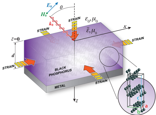
FIG. 1. (Color online). Schematic configuration involving a slab of bulk black phosphorus of thickness d adjacent to a metallic substrate. The black phosphorus layer is exposed to a transverse magnetic field from the vacuum region where the incident electric field is polarized in the x - z plane, and the magnetic field is polarized along y . The incident wavevector \mathbf{k}_0 makes an angle \theta with the z axis. The tensile or compressive strains are applied in the x - y plane and along the z direction (note that the arrows marking applied strain can be reversed corresponding to compressive and tensile strain, respectively). The crystallography principal directions are set as follows: x \equiv a , y \equiv b , and z \equiv c .
