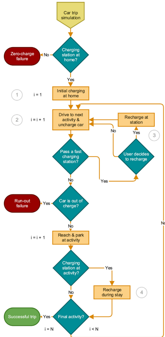
Fig. 2. Steps and decisions during the simulation of a car trip. In this example, the car starts from home and passes N representations of activities and legs. i indicates the current representation. Numbers in circles correspond to the list of steps in this section.
