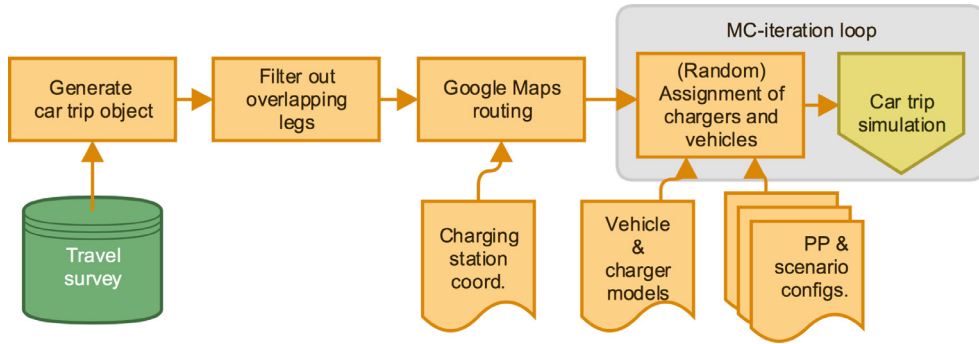
Fig. 1. Overview of the inputs and steps taken by the BEVPO model.
