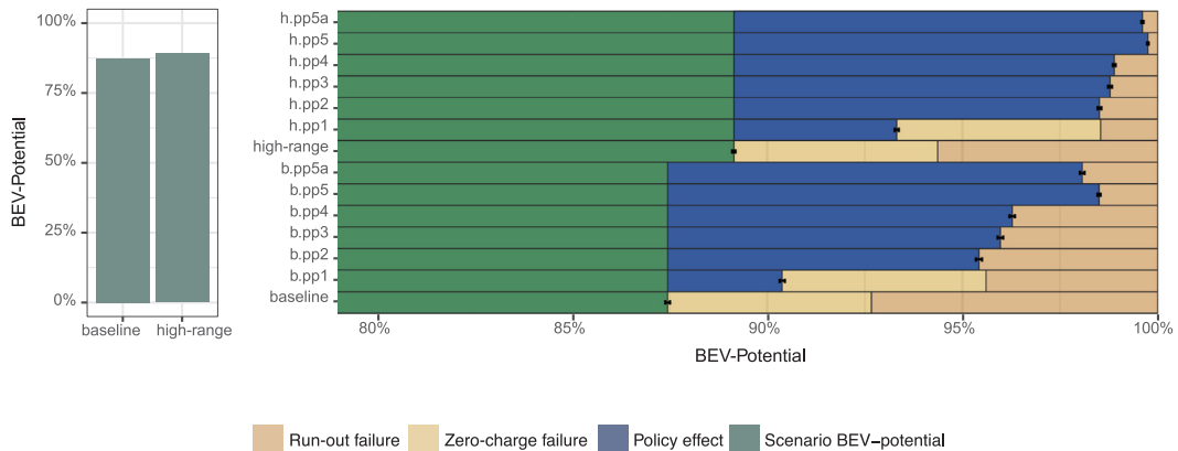
Fig. 3. Simulation results for Switzerland. Left: BEV-potential for the baseline and high-range scenarios. Right: comparison of the policy package effects. pp1–pp5 are cumulative. pp5a is without pp3 and pp4. Error margins indicate variance of the MC-runs.
