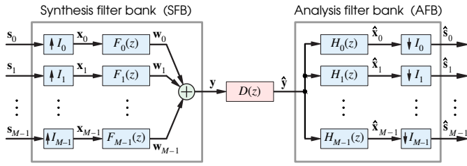
Fig. 1. General M -channel transmultiplexer with configurable sampling rate conversion factors.
