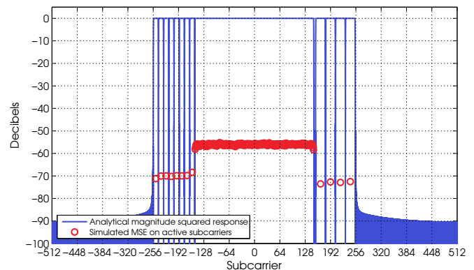
Fig. 5. Analytical magnitude-squared response of the synthesis/analysis FB as well as the simulated MSE on the active subcarriers.
