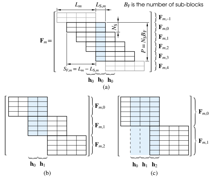
Fig. 3. Structure of block-diagonal synthesis matrix \mathbf{F}_m for L_m = 4 , N = 8 , and L_{S,m} = 1, 2, 3 . The colored columns illustrate the elements of the synthesis matrix that form the shift-variant impulse responses of the synthesis filter bank. (a) For L_{S,m} = 1 , the system has only one impulse response of eight samples. (b) For L_{S,m} = 2 , the system has two eight-samples long responses. (c) For L_{S,m} = 3 , two among the three responses are six samples long and the remaining one is 12 samples long.
