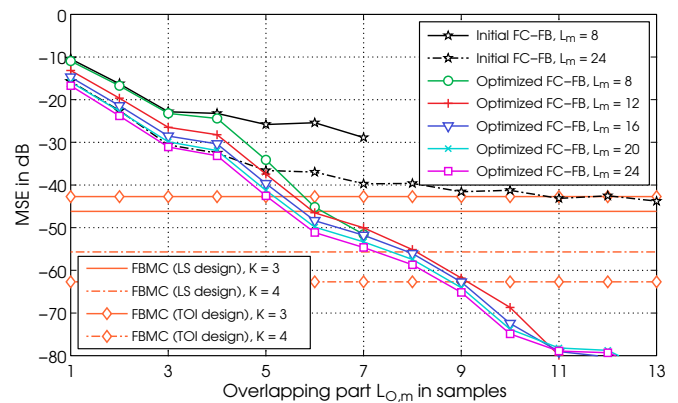
Fig. 4. Simulated MSE as a function of the overlapping part L_{O,m} = L_m - L_{S,m} of the input samples for FC-FB with L_m = 8, 12, 16, 20, 24 . For comparison the MSE of the initial design for L_m = 8 and L_m = 24 as well as the PHYDYAS polyphase FBMC [18] designs with K = 3 and K = 4 are also shown. Here, “LS design” and “TOI design” refer to designs for which the stopband energy and total FB structure based interference, respectively, are minimized [18].
