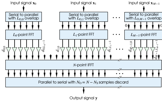
Fig. 2. FC based synthesis FB using overlap-save processing.
