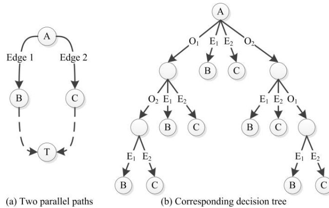
Figure 1. Sequential decisions at a junction of a directed acyclic graph when repeated measurements are noninformative. Prior optimal decisions from nodes B and C to target node T have been solved. In the case of additive objective function, decisions at A are made taking into account the measurement actions and choices of edges A-B and A-C and the optimal objectives B-T and C-T.
