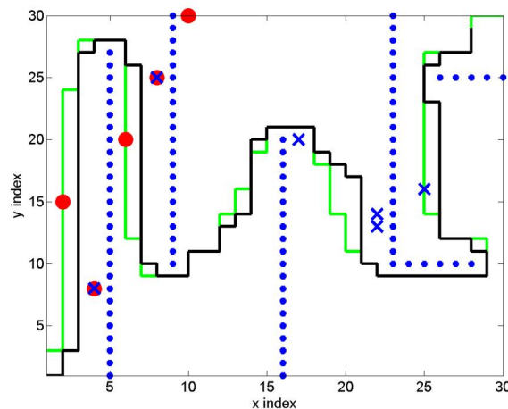
Figure 3. Path planning with a map in the presence of unmapped obstacles. Blue dots: obstacles in the map. Red dots: unmapped obstacles. Blue crosses: observations (true or false) about unmapped obstacles. Green line: optimal path according to known map. Black line: optimal route with optimal sensing for unmapped obstacles.
