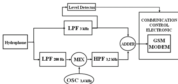
Figure 3. Diagram of frequency shift circuit.
