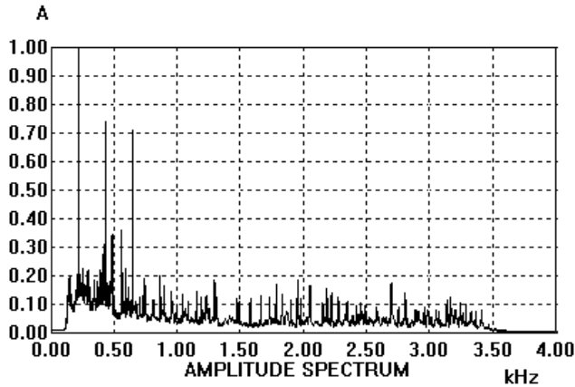
Figure 2. Response of GSM codec RPE-LTP to a modulated signal
