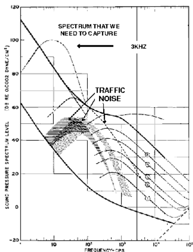
Figure 1. Curves of underwater noise [after 3]
