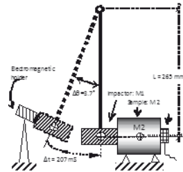
Fig. 1 - Impacting device
