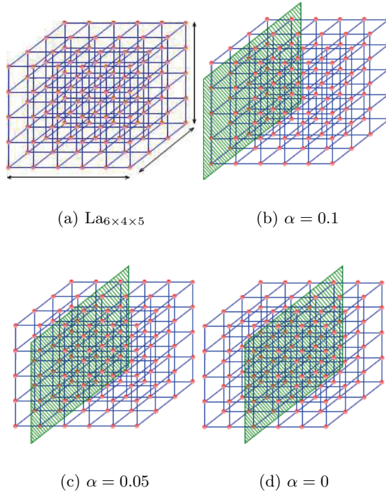
Figure 4: Partitioning of three-dimensional lattice \text{La}_{6 \times 4 \times 5}
