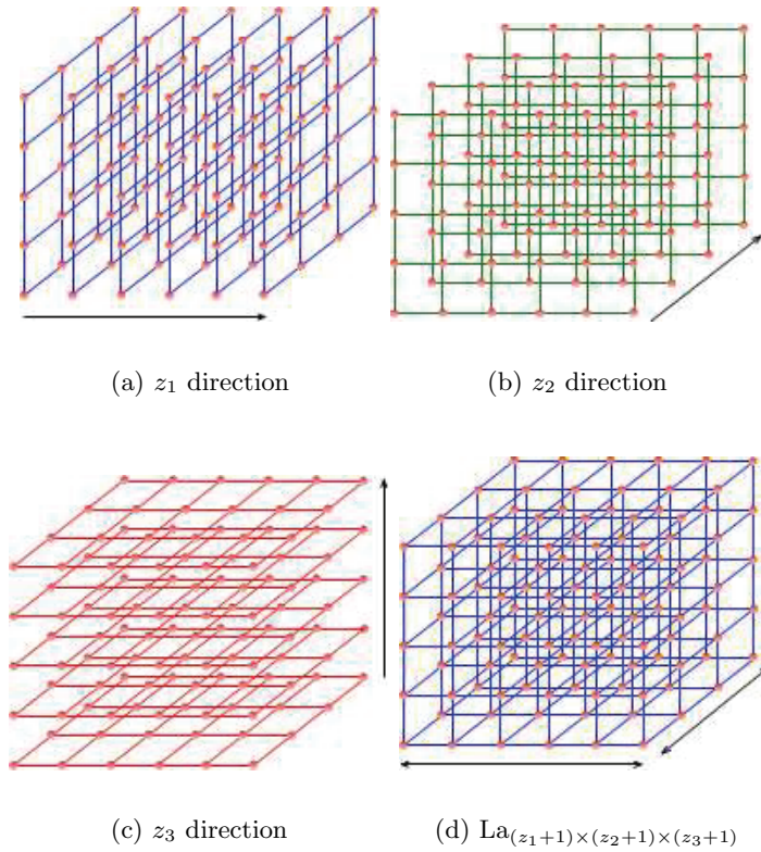
Figure 2: Construction of 3-dimensional lattice
