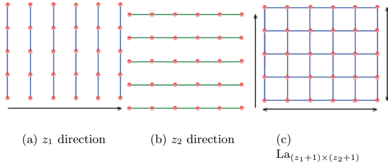
Figure 1: Construction of 2-dimensional lattice
