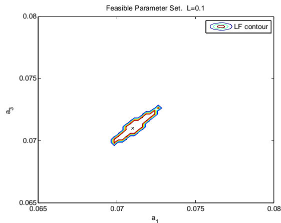
Figure 6. FPS obtained by the likelihood technique in the nonlinear case
