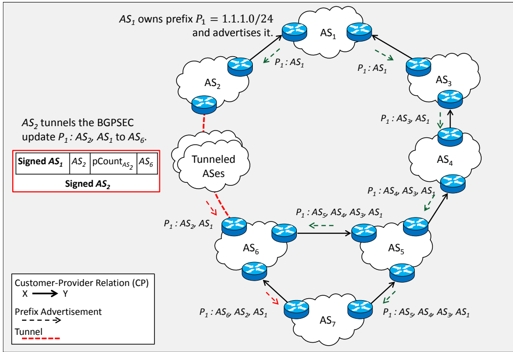
Figure 10: Co-ordinated false AS-Path attack on BGPSEC.
