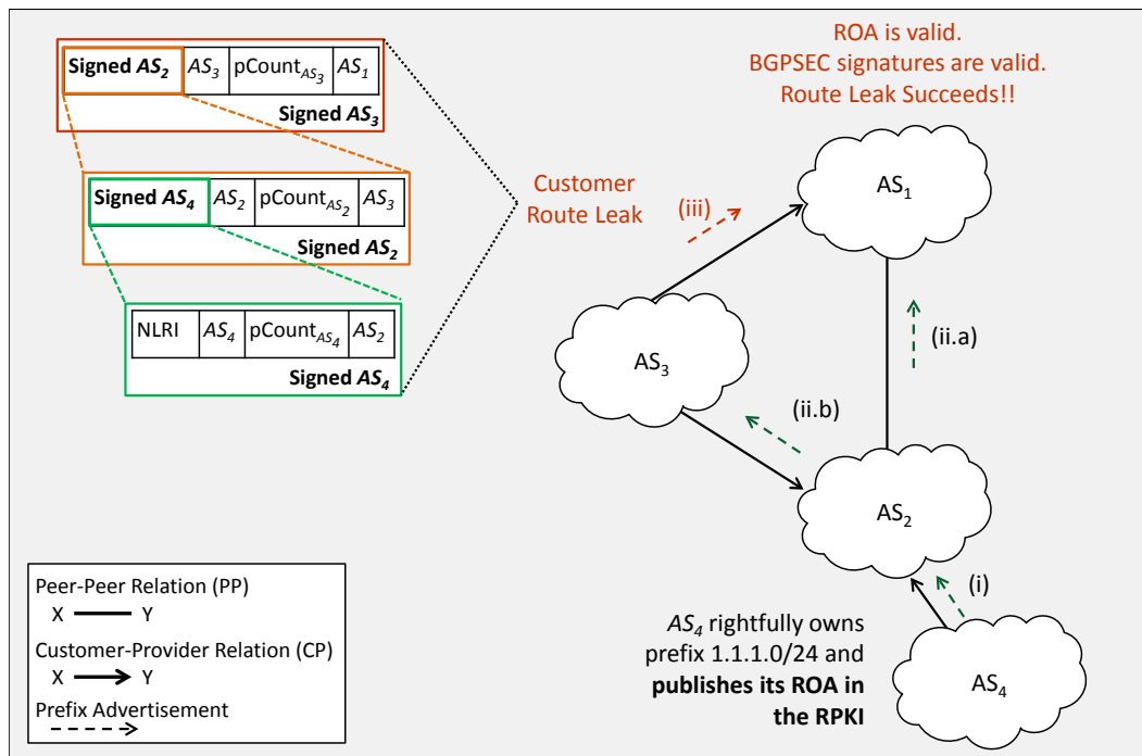
56 Figure 9: Route leak on a customer link in presence of RPKI, ROA and BGPSEC.
