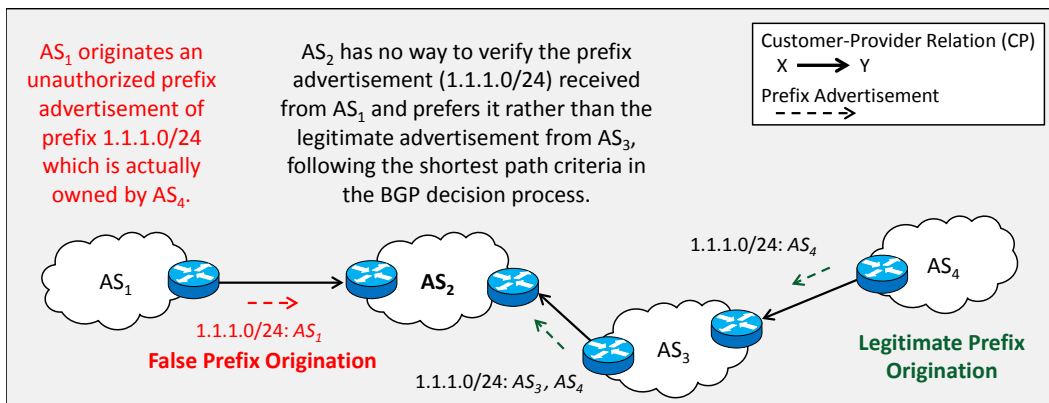
Figure 3: False IP prefix origin attack.
