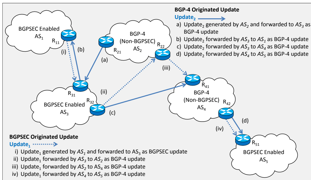
Figure 8: BGPSEC updates in partial deployment scenarios.
