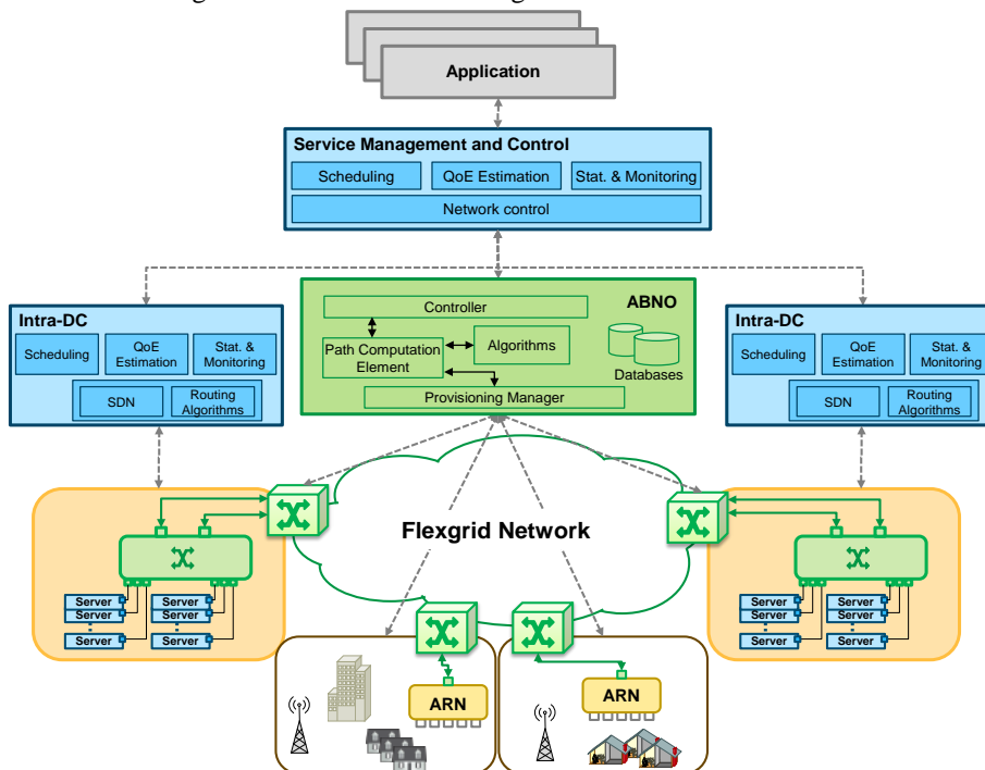
Fig. 3 SHINE's control and management architecture.
