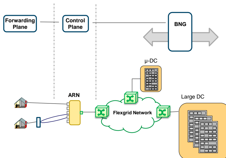
Fig. 6 Fixed broadband access scenario.
