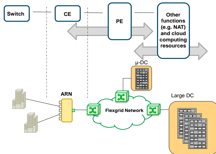
Fig. 4 Business access scenario.
