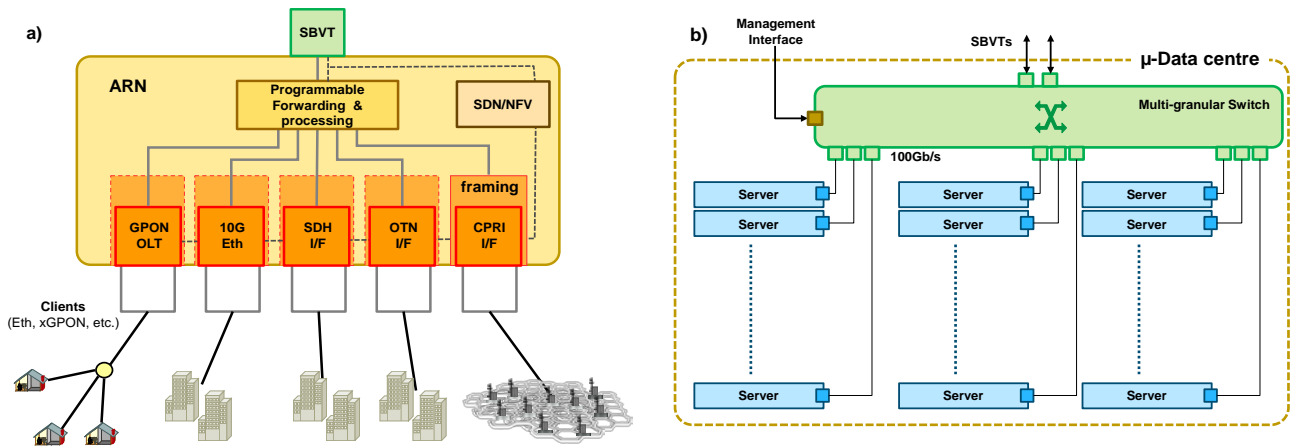
Fig. 2 SHINE's ARN (a) and \mu -DC (b) architecture.
