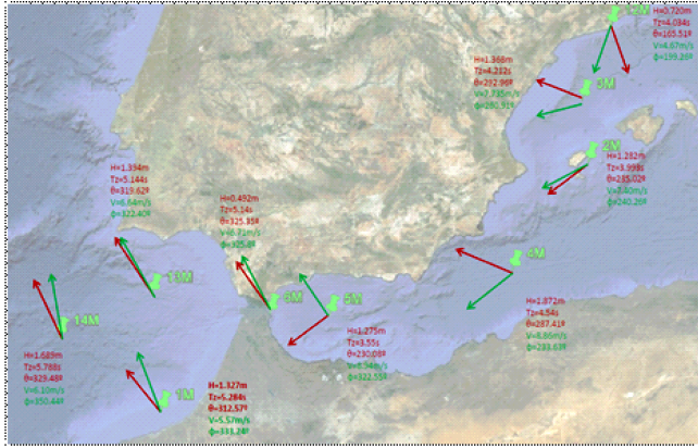
Figure 6: Characteristic map with the illustrate results of the different analyzed points considering Mediterranean and Gibraltar Strait Area
