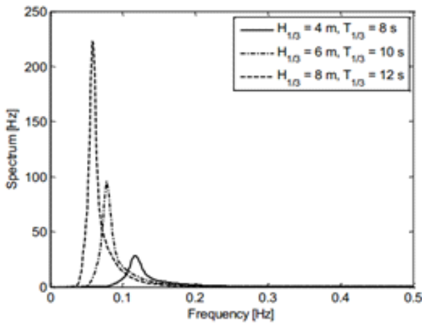
Figure 4: Jonswap Spectrum.
