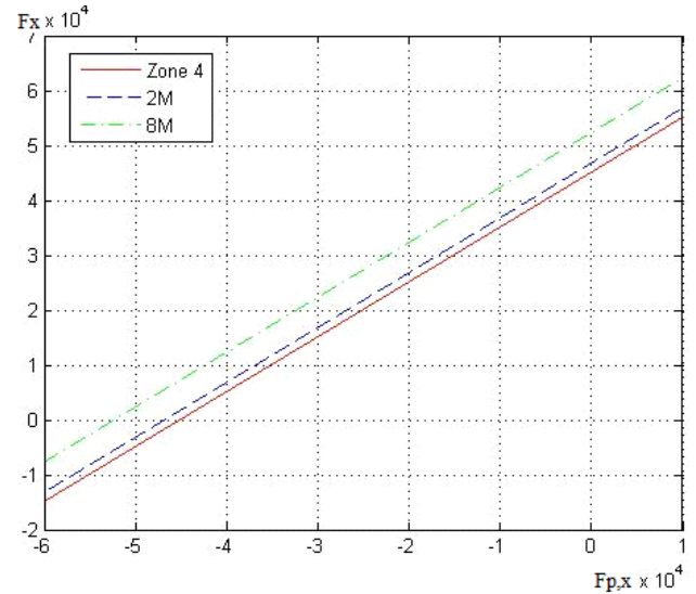
Figure 8: Resultant force on the boat depending on the propulsive force
