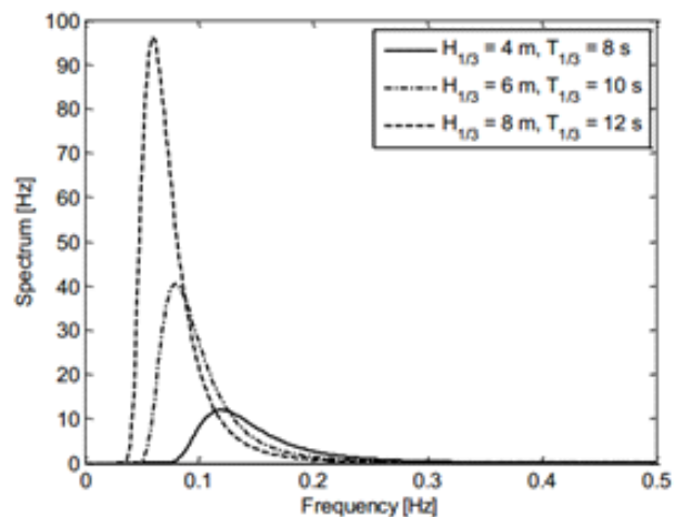
Figure 3: ISSC and Pierson Moskowitz Spectrum.
