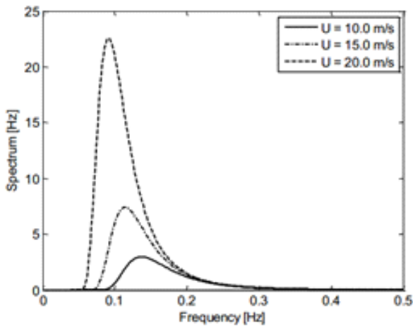
Figure 1: Pierson Moskowitz Spectrum
