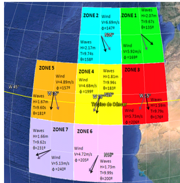
Figure 5: Characteristic map with the illustrate results of the seven analyzed zones from North Atlantic Ocean
