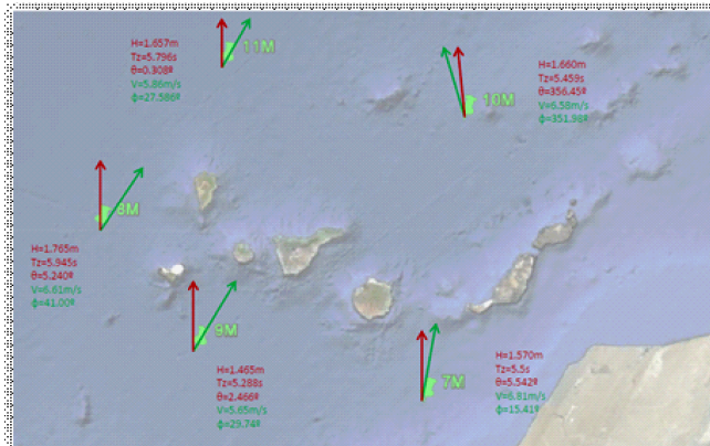
Figure 7: Characteristic map with the illustrate results of the different analyzed of different points considering Canary Area
