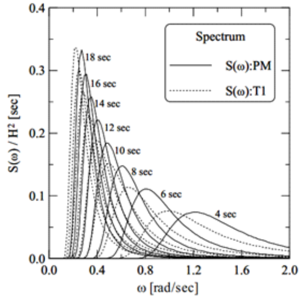
Figure 2: ISSC and Pierson Moskowitz Spectrum.
