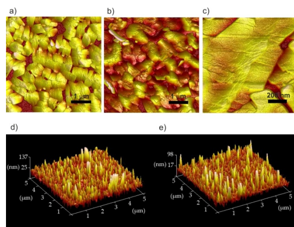
Fig. 6 AFM images of vacuum-deposited 3 films deposited on a) bare SiO 2 (5 × 5 μm 2 ), b) polystyrene treated SiO 2 (5 × 5 μm 2 ) and c) polystyrene treated SiO 2 (1 × 1 μm 2 ). AFM images of vacuum-deposited 4 films deposited on d) bare SiO 2 (5 × 5 μm 2 ) and e) polystyrene treated SiO 2 (5 × 5 μm 2 ).
