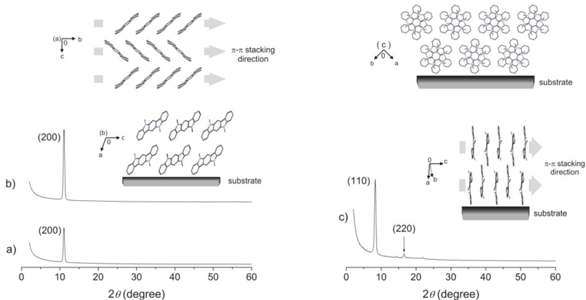
Fig. 5 GIXRD pattern of vacuum-deposited 3 films on a) bare and b) polystyrene-treated c-Si/SiO 2 surfaces. The inset image shows the molecular packing of compound 3 with the (100) plane situated at 27° (above) and perpendicular (below) to the paper plane, respectively. c) GIXRD pattern of vacuum-deposited 4 film on polystyrene treated c-Si/SiO 2 surface. The inset images show the molecular packing in the thin films seen from two different perspectives, being the (110) plane situated perpendicular to the paper. The hydrogen atoms were omitted for clarity.
