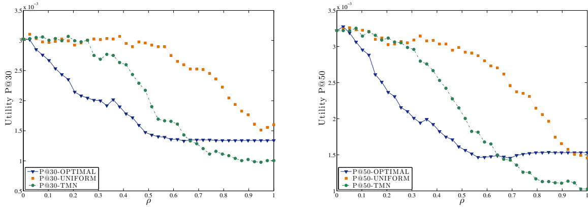
(a) Average value of utility P@30 calculated for different values of \rho . (b) Average value of utility P@50 calculated for different values of \rho .
