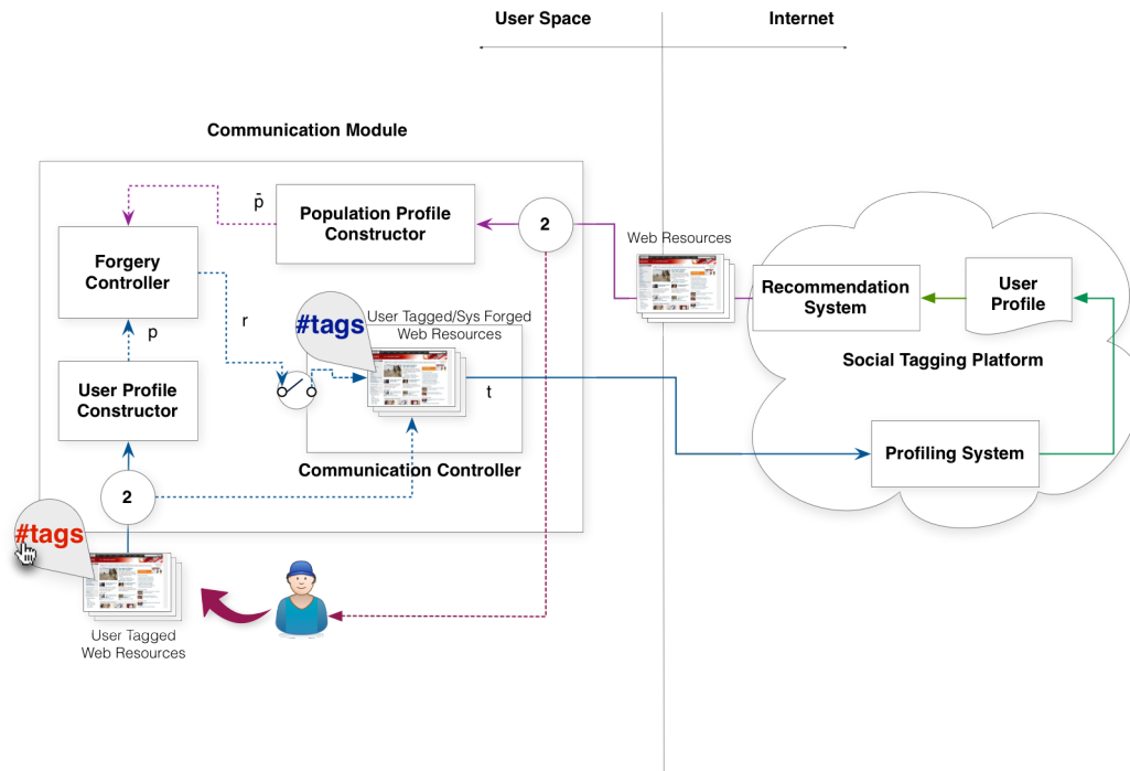
Figure 2: The proposed architecture of a communication module managing the user data flows with a social tagging platform and implementing different possible forgery algorithms.
