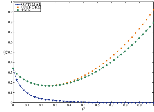
(b) Privacy risk \mathcal{R} against forgery rate \rho for a single user.
