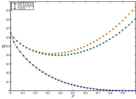
(a) Privacy risk \mathcal{R} against forgery rate \rho for all users.
