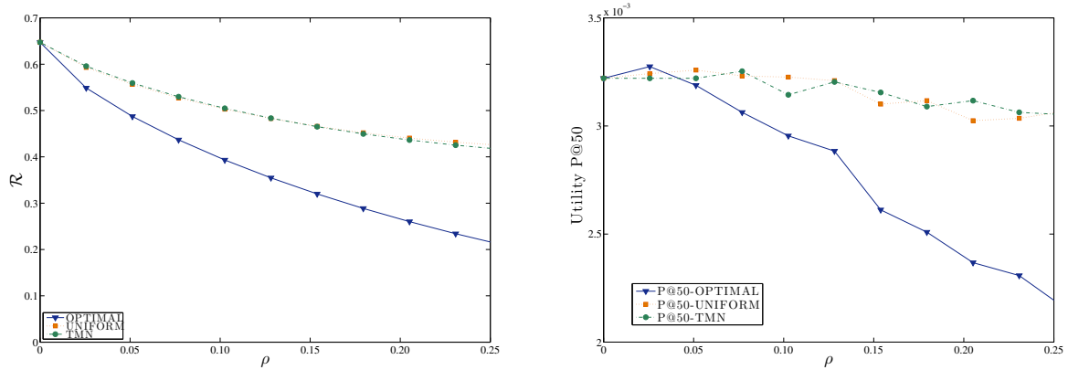
(a) Privacy risk \mathcal{R} against forgery rate \rho for all users applying a PET considering only values of \rho \leq 0.25 . (b) Average value of utility P@50 calculated for different values of \rho \leq 0.25 .
