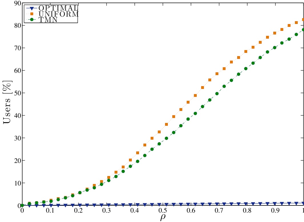
Figure 7: Actual number of users increasing their privacy risk as a side effect of applying a certain strategy for a given value of \rho .
