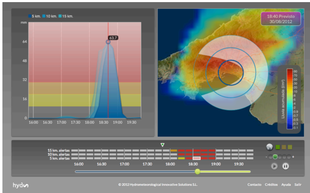
Figure 6. Example of the viewer interface for the Palma de Mallorca point 50 minutes before the storm hit the city (18:40h August 30 th , 2012). The left panel shows the evolution of the 30 min. accumulation for the three intelligent areas surrounding the point and the right panel shows the accumulation field and the intelligent area. Bottom bar shows the warnings according to defined thresholds.
