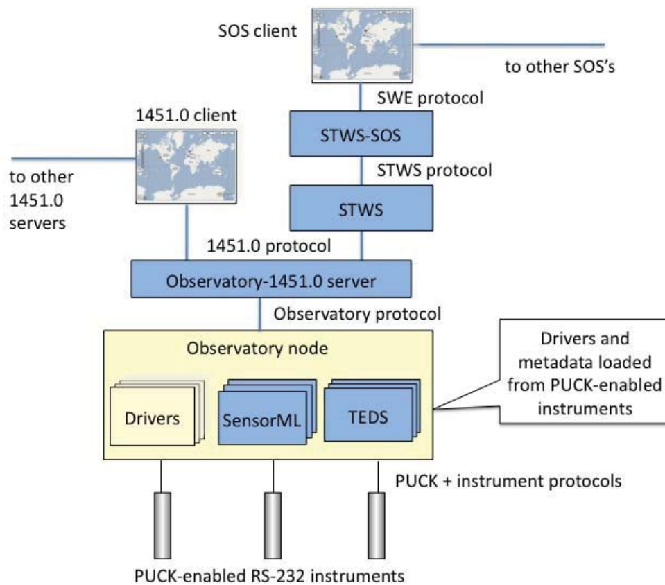
Figure PUCK-1: Basic architecture of PUCK-1451-SWE test-bed
