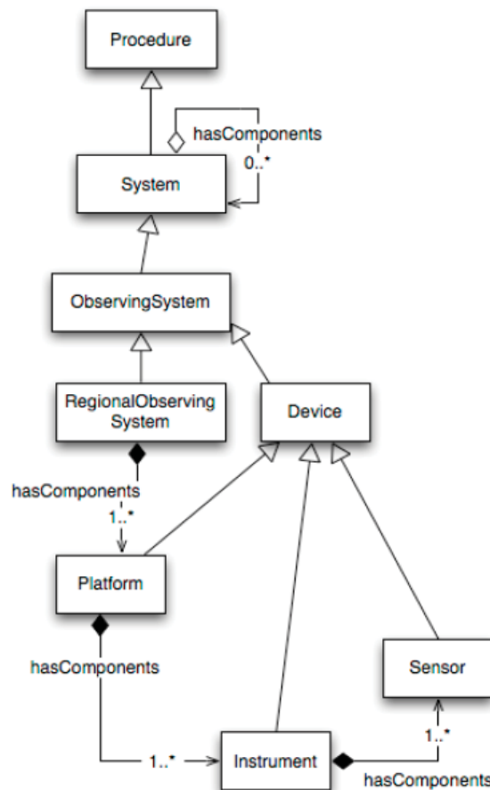
Figure [Complex Systems-1]. Simple UML for systems components. The top classes depict the SensorML conceptual model where a system is a procedure. And a system has components.
