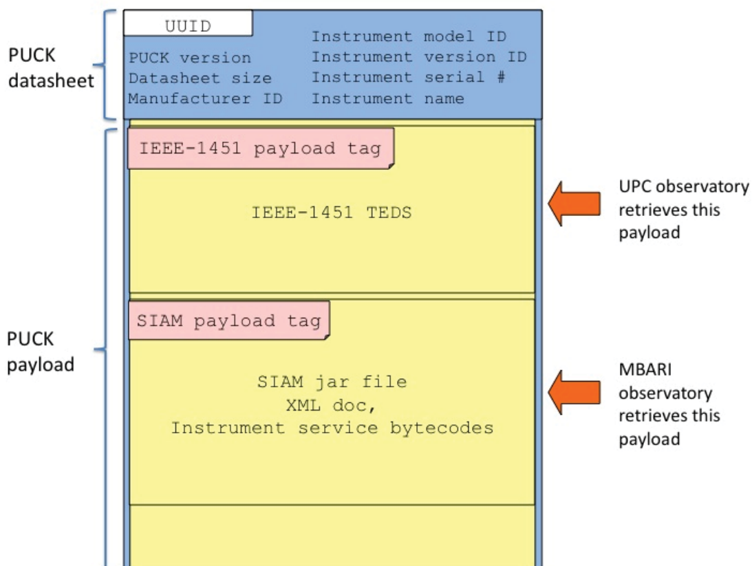
Figure PUCK-4: PUCK memory map example showing multiple “tagged” payload components
