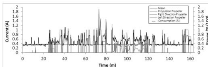
Consumption of the vehicle versus power of the propellers
