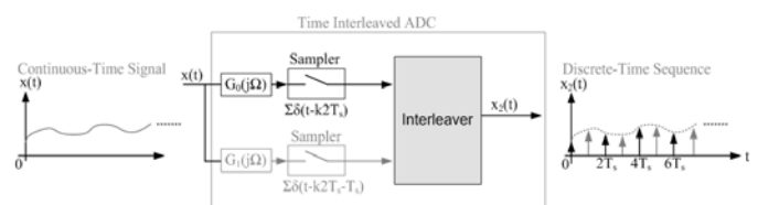
2-channel TI-ADC with frequency response mismatch
