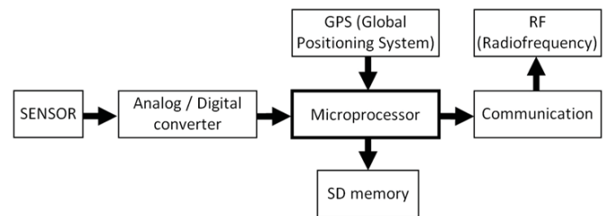
Block diagram of the acquisition system
