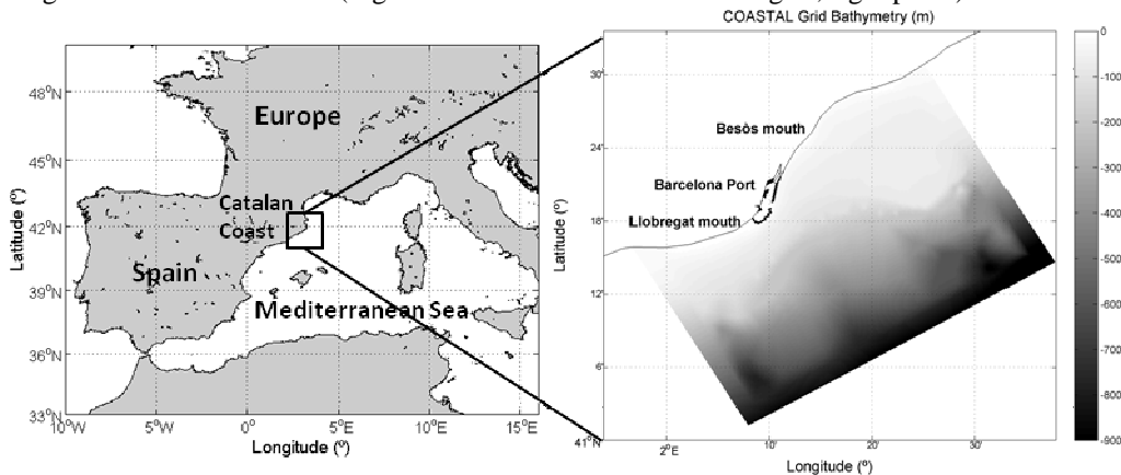
Figure 1. Catalan Coast and coastal grid
