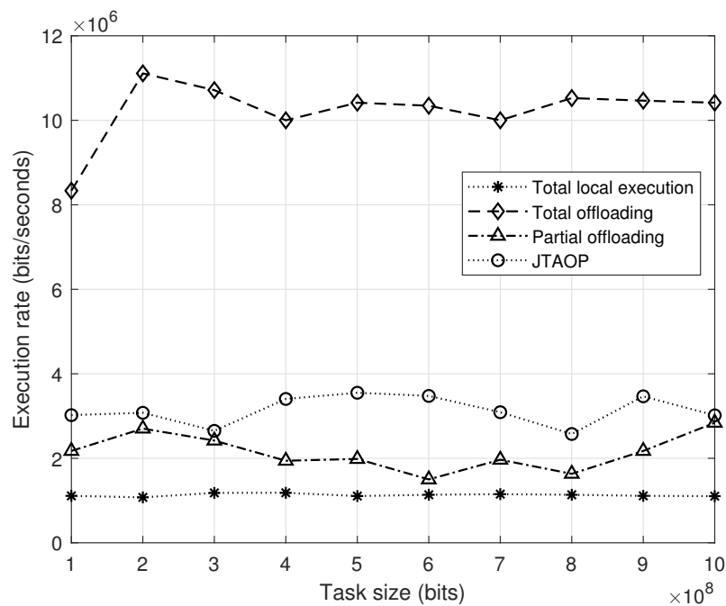
Figure 6. Execution rate vs. task size.
