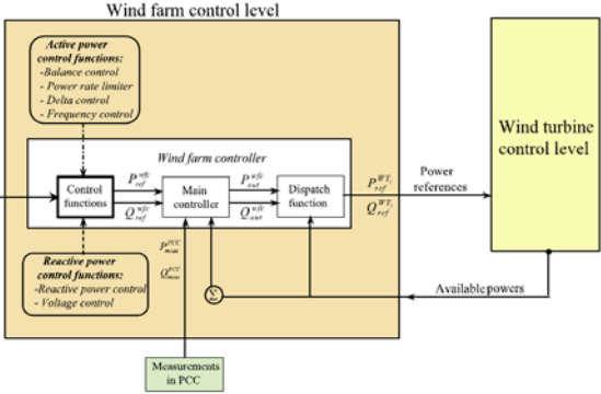
Fig. 10. WPP main controller [8].
