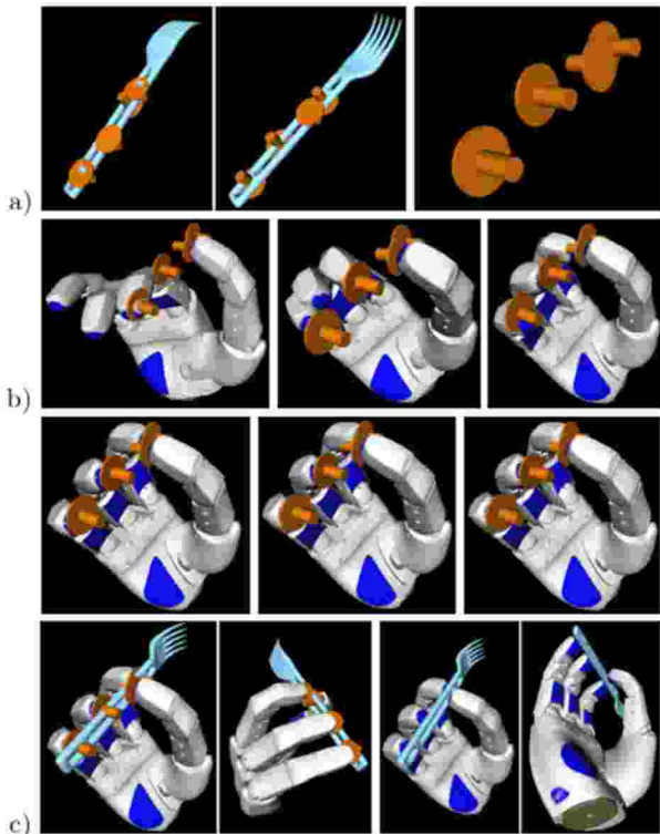
Fig. 6. a) The desired contact points with and without the fork (the position and orientation constraints are given by the center of each disk and the attached cylinder respectively); b) The initial hand configuration (first image) and the the hand configurations obtained in the next five jacobian iteration; c) Views of the final grasp configuration after 6 jacobian iterations (the first two images remark the contact points).
