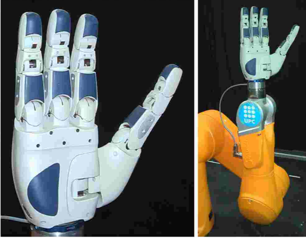
Fig. 1. Mechanical hand SAH assembled on an industrial robot arm.
