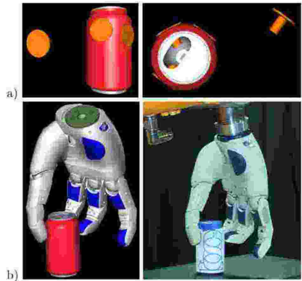
Fig. 8. a) Two views of the contact constraints on a can, and, b) obtained solution in simulation, and execution of the solution with the real hand SAH.
