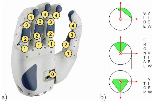
Fig. 2. a) Hand and finger joints; b) Contact region on the fingertip surface.
