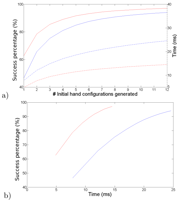
Fig. 9. Statistical performance of the approach. Red lines correspond to results obtained with initial hand configurations obtained with the proposed off-line work (Section 3.2), and blue lines to results obtained with random initial hand configurations: a) Success percentage (continuous lines) and execution time (dashed lines) vs. the number of initial configurations generated; b) Success percentage vs. execution time.
