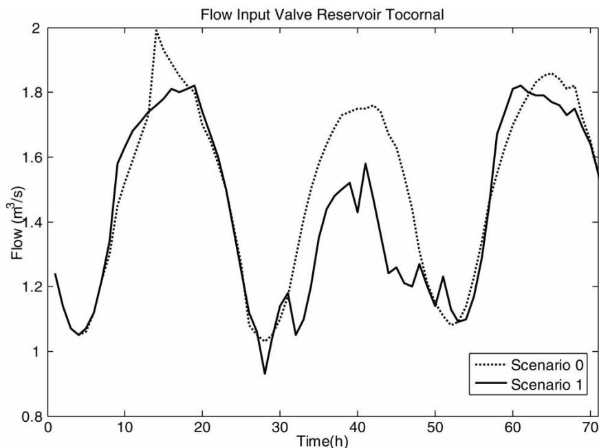
Figure 7 | Flow at the Input Valve of Tocornal Reservoir.
