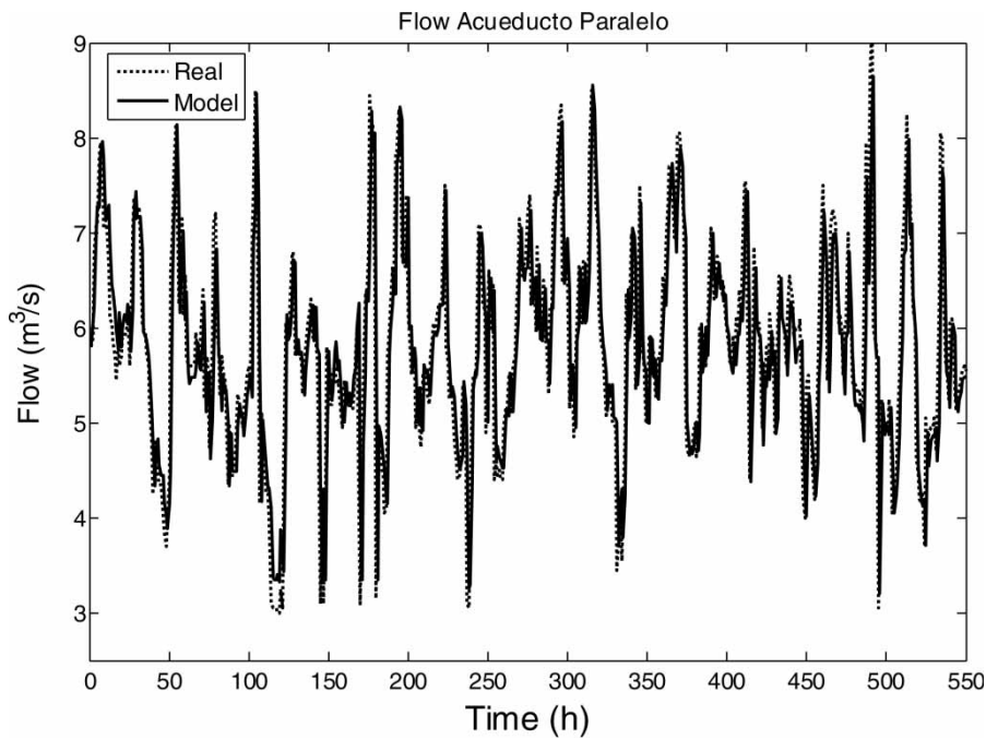
Figure 3 | Modelled vs. real downstream flow at Acueducto Paralelo.
