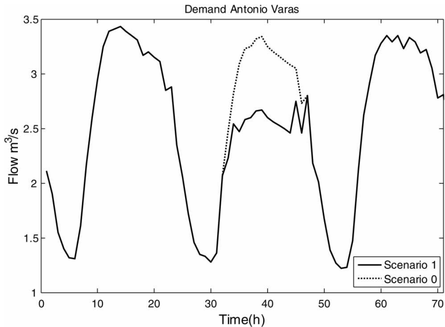
Figure 4 | Demand curve at a Antonio Varas consumer area.
