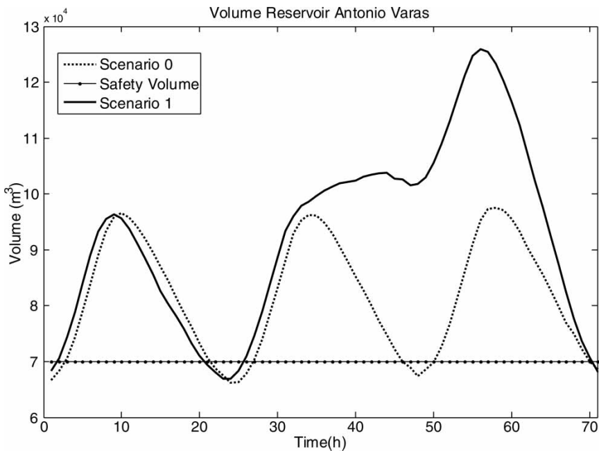
Figure 6 | Volume at the Antonio Varas Reservoir.
