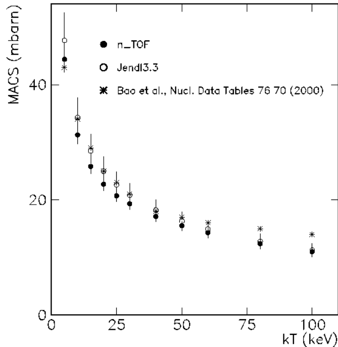
Figure 1: Comparison of MACS calculated from our ^{90}\text{Zr} data (full circles), with values obtained from JENDL3.3 (open circles) and the compilation of Ref.[2] (asterisks).
