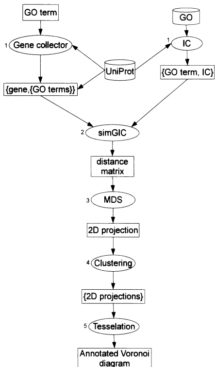
Fig. 1. A diagram of the proposed algorithm. Ellipses represent methods, rectangles represent data and cylinders represent external data sources.
