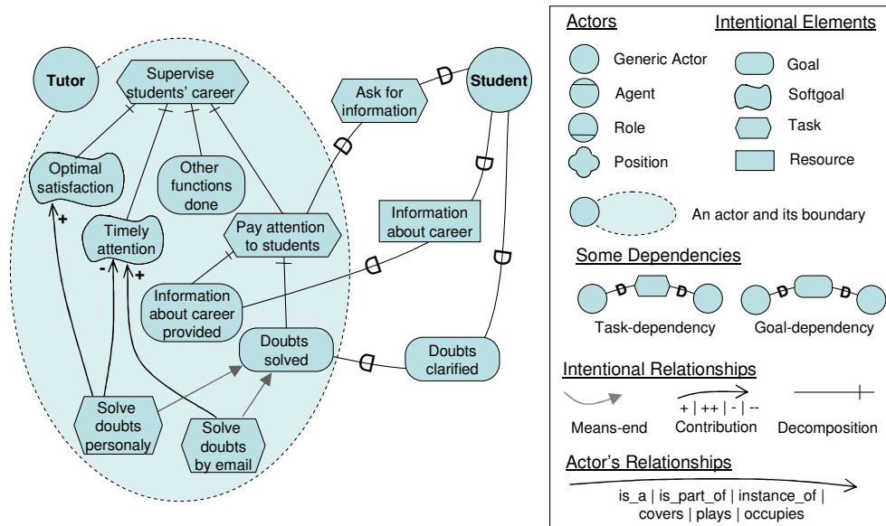
Fig. 2. The i* framework: an example on tutoring.
