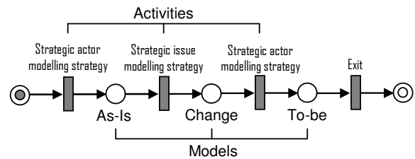
Fig. 1. Kavakli's view of the i^* scope into GORE processes
