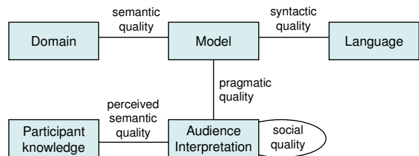
Fig. 5. The second version of SEQUAL (1995) [25]
