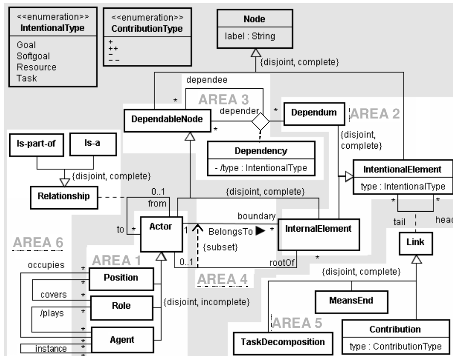
Fig. 3. Core concepts of i*
