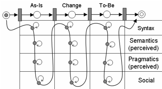
Fig. 7. The space of qualities to measure
