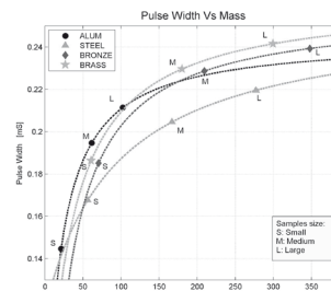
Fig. 2. Pulse-width Vs mass. Hard markers are known experimental results. Dotted lines are curve fitting results.
