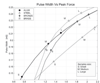
Fig. 3. Pulse-width Vs Peak Force. Hard markers are known experimental results. Dotted lines are curve fitting results.
