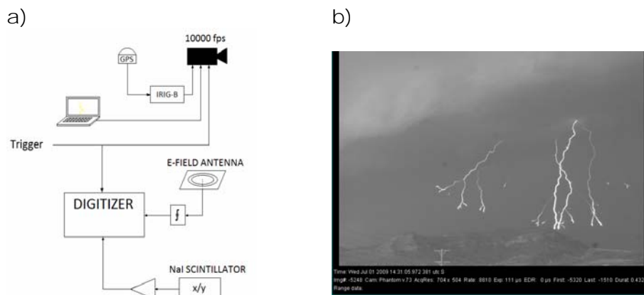
Figure 1. a) Scheme of the instrument; and b) frame of several downward leaders to ground of the same flash.
