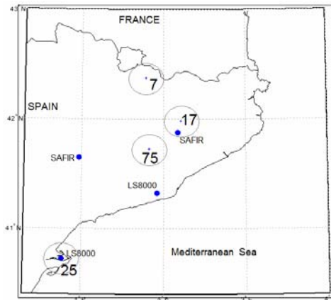
Figure 2. Locations of the SAFIR and LS8000 sensors (blue filled circles) and the observation sites (grey circles with numbers). The numbers in the circles indicates the number of VHF sources per flash observed in the region.
