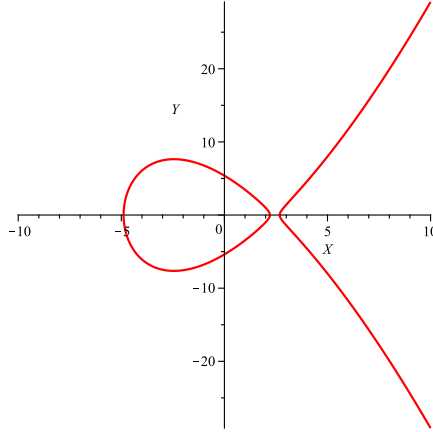
Figure 1: The elliptic curve Y^2 = X^3 - \frac{1288423179}{71639296} X + \frac{8775405707427}{303177500672} .
