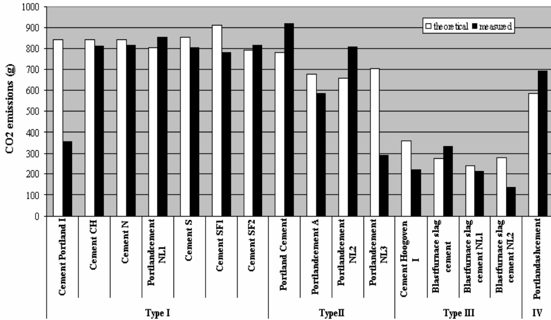
FIGURE 2: Comparison of total CO 2 emissions according to the theoretical model and total given in the inventory for each cement type
