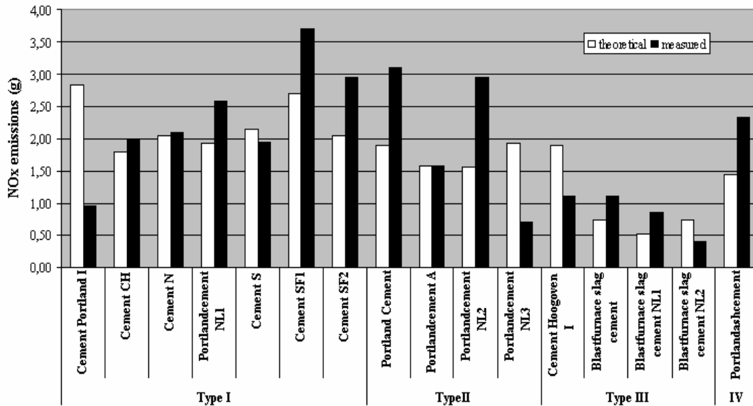
FIGURE 3: Comparison of total NO x emissions according to the theoretical model and total given in the inventory for each cement type
