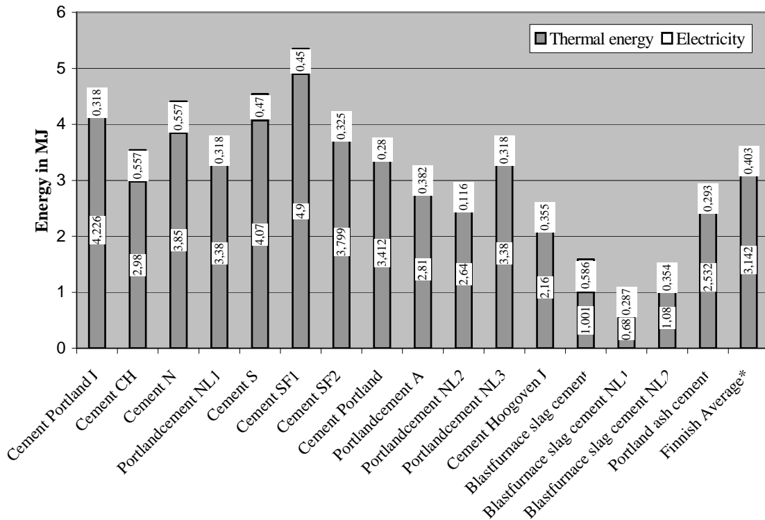
FIGURE 1: Energy consumption (in MJ) for the production of 1 kg of cement (electricity and thermal energy)
