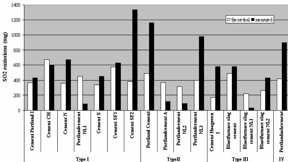
FIGURE 4: Comparison of total SO 2 emissions according to the theoretical model and total given in the inventory for each cement type
