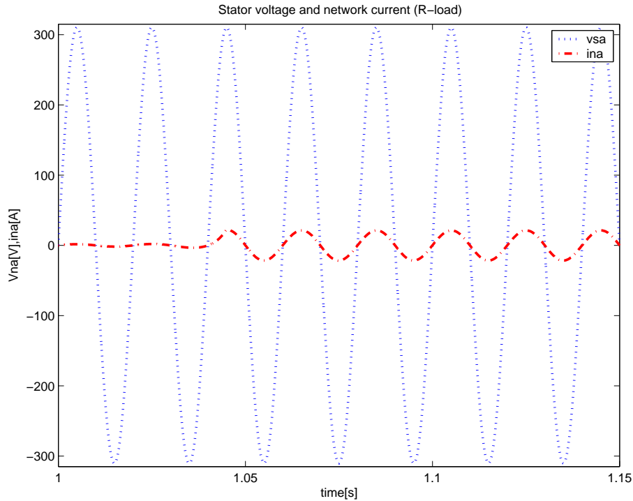
Figure 5: Network voltage and current ( v_{sa} , i_{na} ) for a resistive load.
