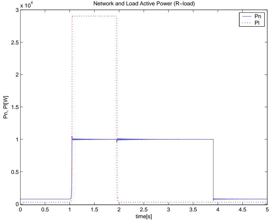
Figure 3: Network and load active powers ( P_n , P_l ) for a resistive load.
