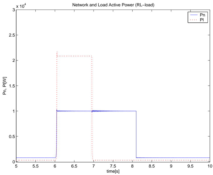
Figure 8: Network and load active powers ( P_n , P_l ) for an RL load.
