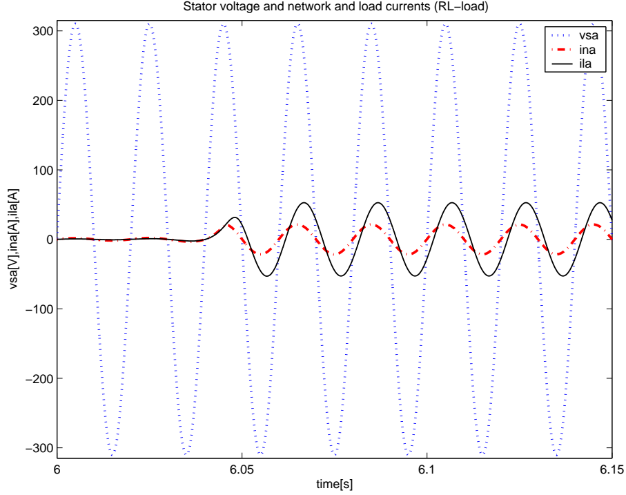
Figure 6: Network voltage ( v_{sa} ) and network and load currents ( i_{na} , i_{la} ) for an RL load.
