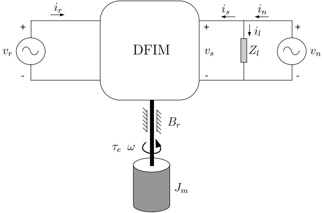
Figure 1: Doubly fed induction machine, flywheel, power network and load.
