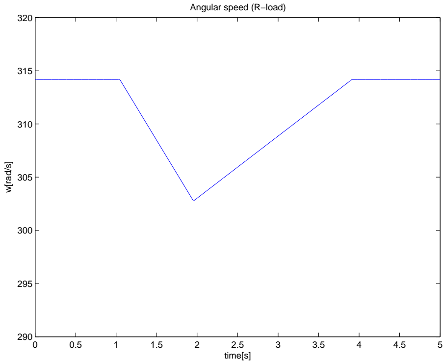
Figure 4: Angular speed ( \omega ) for a resistive load.
