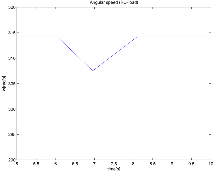
Figure 7: Angular speed ( \omega ) for an RL load.
