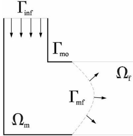
Figure 7: Lost foam casting: Problem setting.
