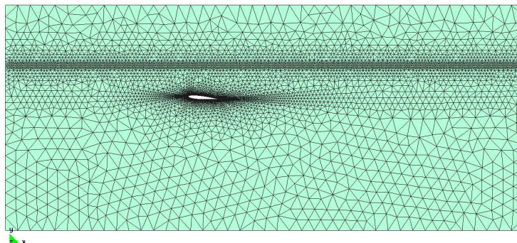
Figure 10: Mesh around the NACA profile.
