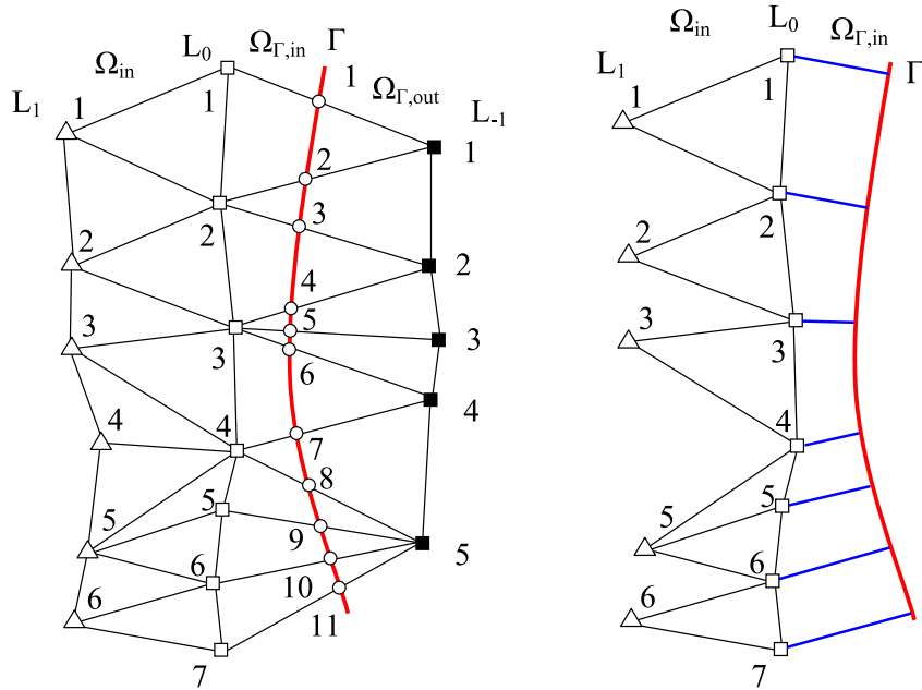
Figure 3: Immersed boundary sketch (left) and domain of extrapolation (right) in a 2D example
