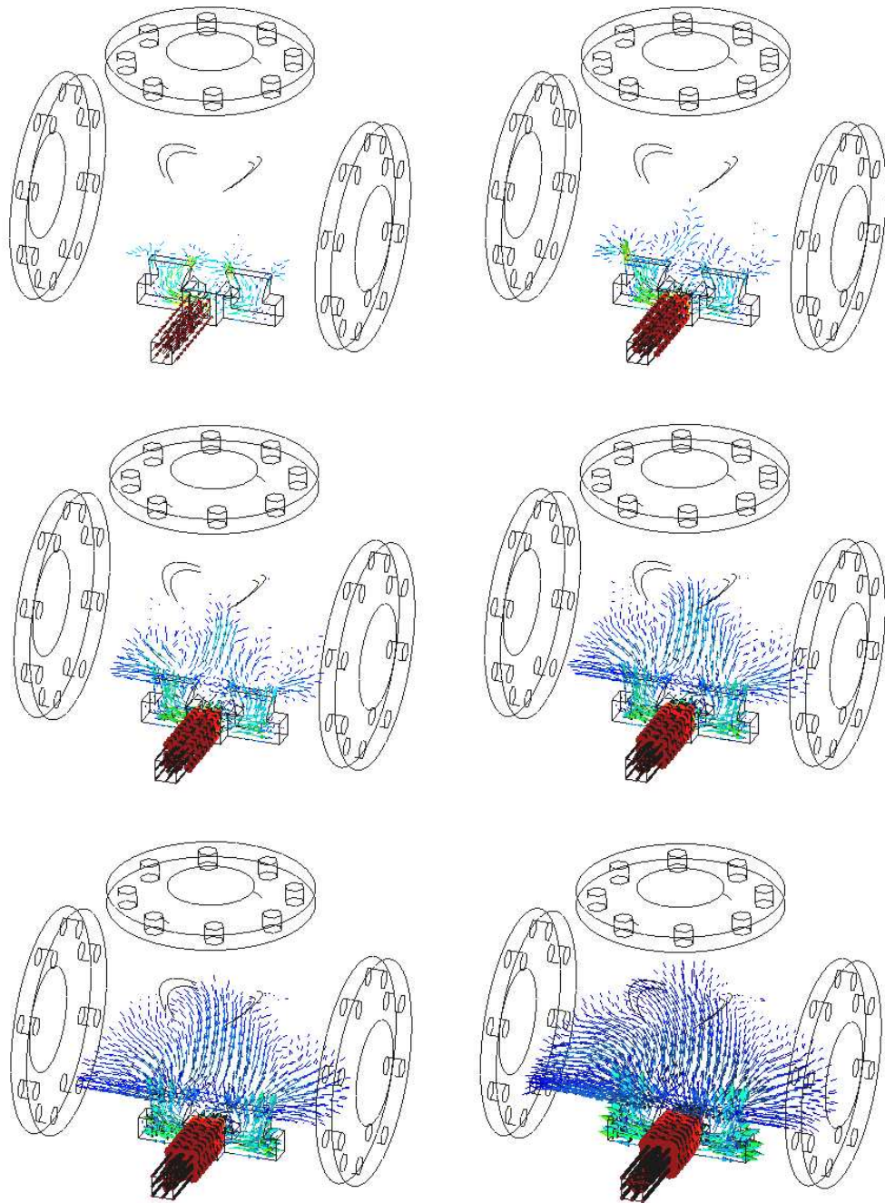
Figure 9: Velocity vectors for the lost foam casting example.
