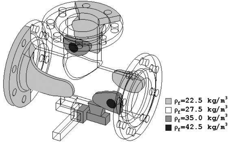
Figure 8: Geometry and foam density for the lost foam casting example.
