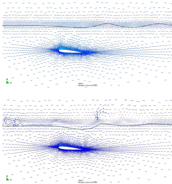
Figure 12: Velocity field and free surface shape at t = 6 . Free surface model (top) and two phase model (bottom).
