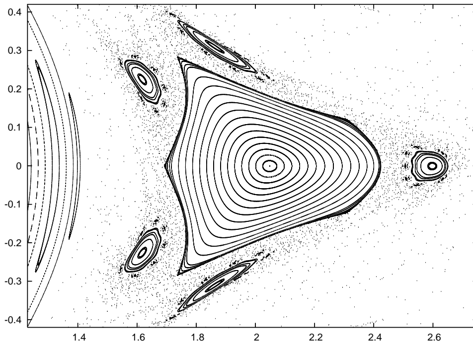
FIG. 4.5. Poincaré section for e = 0.1 (Figure: Sergi Simon)
