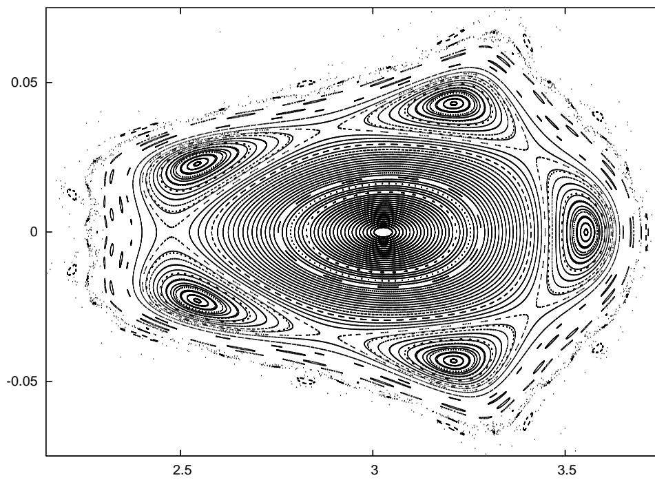
FIG. 4.6. Poincaré section for the Sitnikov problem, e = 0.4 (Figure: Sergi Simon)
