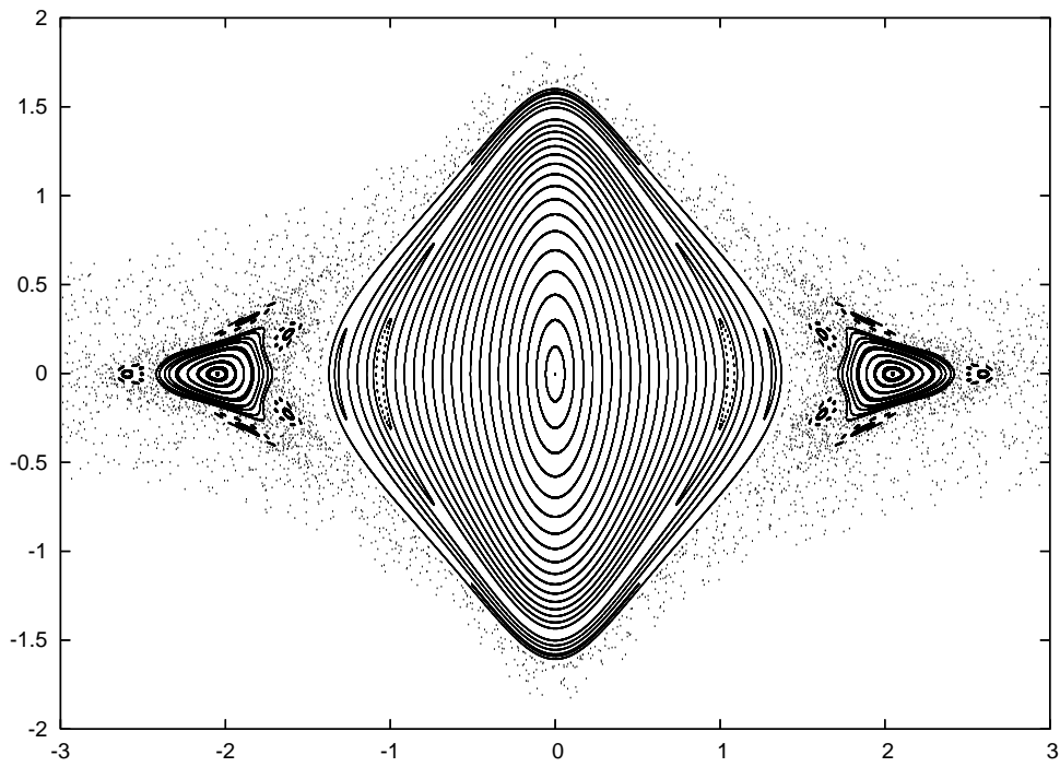
FIG. 4.4. Poincaré section \sin q_2 = 0 for the Sitnikov problem, e = 0.1 (Figure: Sergi Simon)
