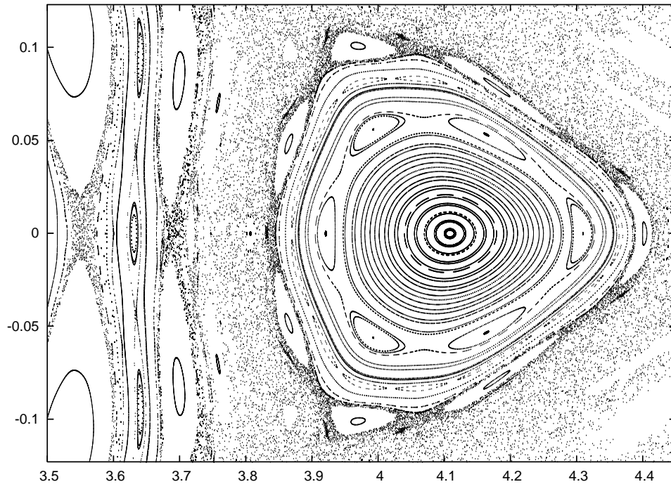
FIG. 4.3. Poincaré section for e = 0.01 (Figure: Sergi Simon)
