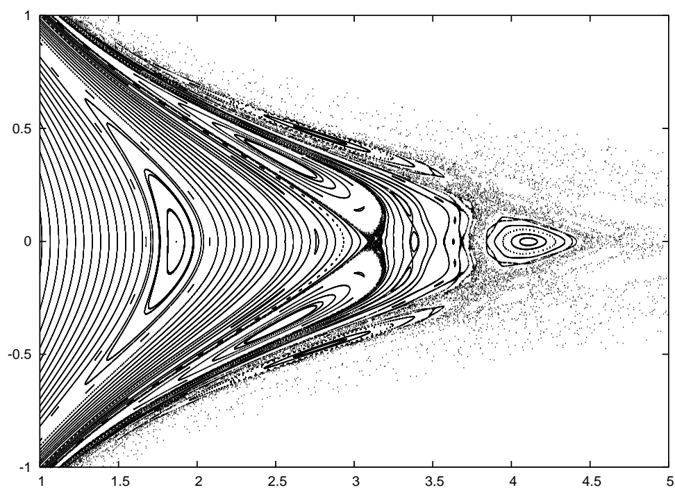
FIG. 4.2. Poincaré section \sin q_2 = 0 for the Sitnikov problem, e = 0.01 (Figure: Sergi Simon)
