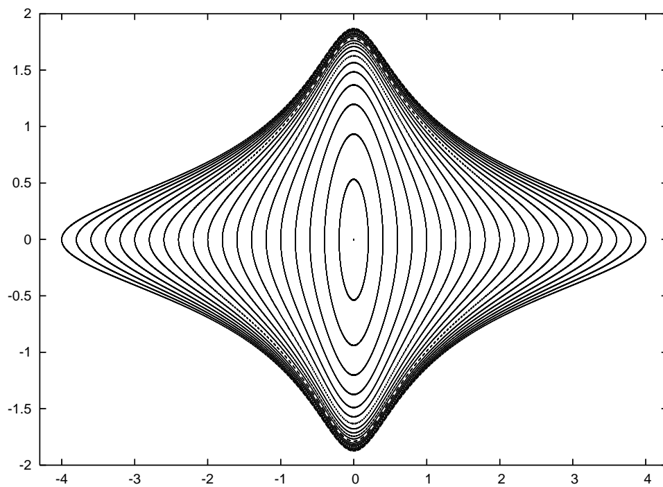
FIG. 4.1. Poincaré section \sin q_2 = 0 for the Sitnikov problem: e = 0 (Figure: Sergi Simon)
