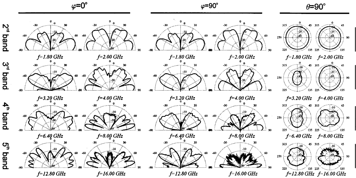
Fig. 5. Radiation pattern for the 30^\circ Sierpinski monopole.
