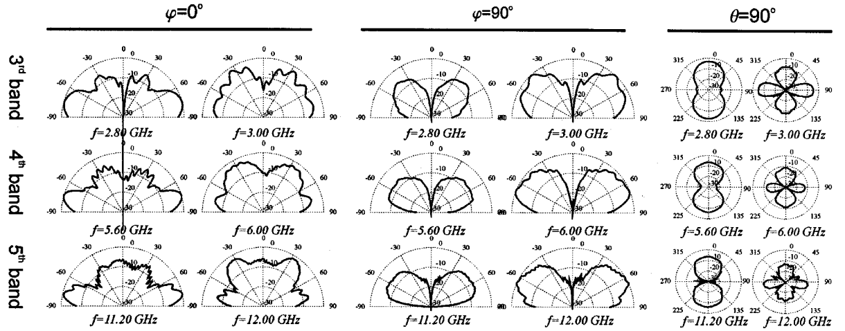
Fig. 4. Radiation pattern for the 90^\circ Sierpinski monopole.
