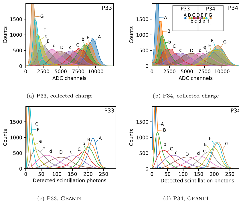
Fig. 5. Scintillation-light sharing. Horizontal scan from P33 to P34 using the 1 mm diameter FWHM 2.0 Å neutron beam in 0.5 mm steps. The colors and beam locations are presented in the key (inset, top right panel) which applies to both the measured gain-corrected charge distributions (filled histograms, top panels) and the GEANT4 simulations of the scintillation-light yields (open histograms, bottom panels). Spectra for positions a and f are not shown as they are almost identical to the spectra obtained at the adjacent positions. (For interpretation of the references to color in this figure legend, the reader is referred to the web version of this article.)
