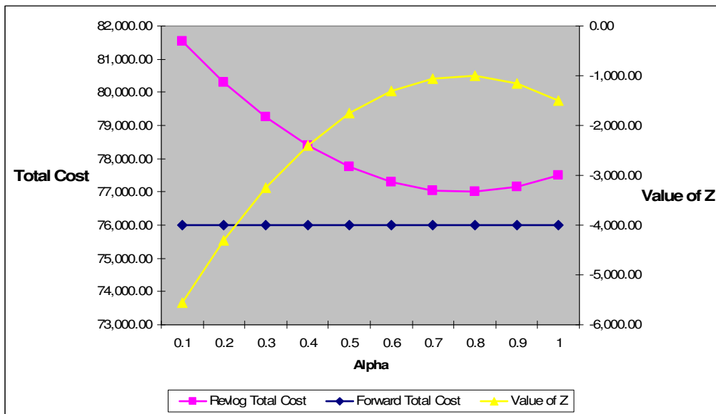
Fig. 3. Model with constant capacity costs: Total Costs for \delta^*
