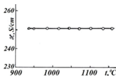
Figure 1: The temperature dependence of the conductivity of an individual DM.
