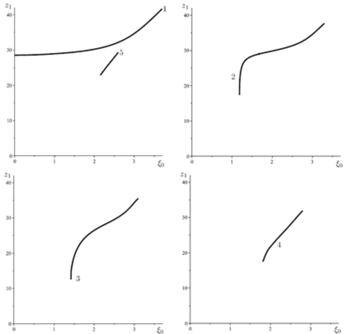
Figure 4: Dependences z_1 = z_1(\xi_0) for 1) \Delta p = 0 Pa; 2) \Delta p = 0.1 Pa; 3) \Delta p = 1 Pa; 4) \Delta p = 2 Pa; 5) \Delta p = 3 Pa in case of wetting.
