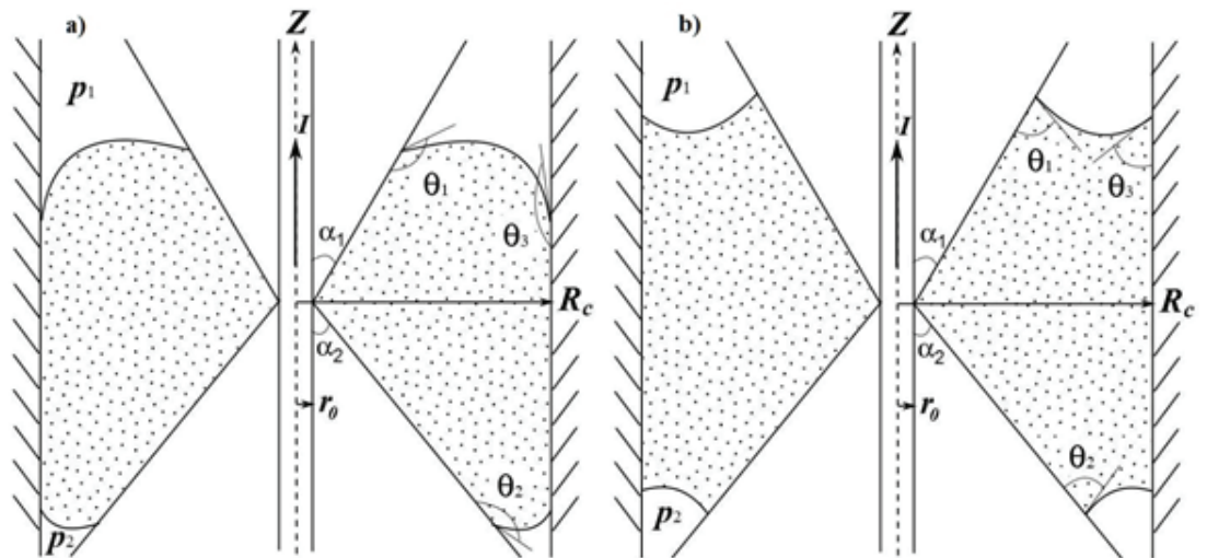
Figure 1: Ferrofluid valve between coaxial conical and cylindrical surfaces in the magnetic field of a straight current-carrying wire under a pressure drop in case of (a) non-wetting and (b) wetting.
