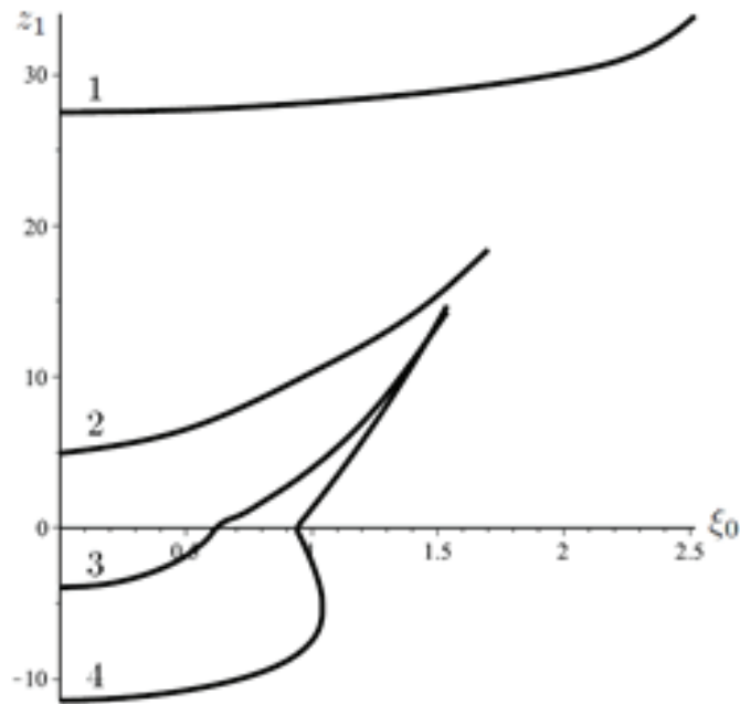
Figure 2: Dependences z_1 = z_1(\xi_0) for 1) \Delta p = 0 Pa; 2) \Delta p = 10 Pa; 3) \Delta p = 20 Pa; 4) \Delta p = 100 Pa in case of non-wetting.
