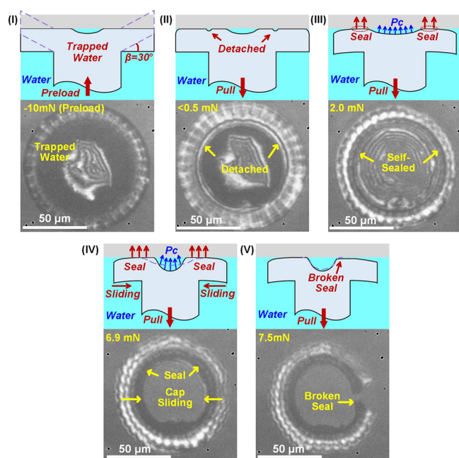
Figure 4. Image sequence illustrating the underwater detachment of the 30° cupped microstructure. Optical micrographs show the contact zone, while illustrations represent side views to depict underlying mechanisms: (I) initial contact of the cupped microstructure upon compressive preloading of the cup (dashed lines for the undeformed state). (II) The structure partially detaches while water starts to flow into the contact. (III) The hydrostatic pressure, p_c , of the entrapped water underneath the contact decreases, leading to seal formation. (IV) The sealed contact shrinks by inward sliding of the seal. (V) The seal breaks by inward collapse of the cup just before detachment. Scale bars: 50 \mu\text{m} .
