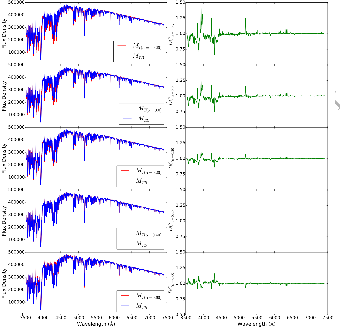
Figure 10. Example differential corrections, which are applicable for MILES star m0067 (=HD010700: T_{\text{eff}}=5264\text{K} , \log g=4.36 , [\text{Fe}/\text{H}]=-0.50 , [\text{Mg}/\text{Fe}]=0.40 ). The left panel compares the resulting spectra of theoretical enhanced (or deficient) ( M_{T(\alpha=x)} ) and theoretical base M_{TB} stars. In these plots ( \alpha=x ) is short for ([\alpha/\text{Fe}]=x) . Flux Density is in units of \text{erg}/\text{s}/\text{cm}^2/\text{\AA} . The right panel shows the resulting differential correction ( DC_{(\alpha=x)} ), derived from equation (7), for each of the output [\alpha/\text{Fe}] abundances. Note that for this star, the differential correction for [\alpha/\text{Fe}]=0.40 is 1, because the empirical MILES star is already at [\text{Mg}/\text{Fe}]=0.40 .
