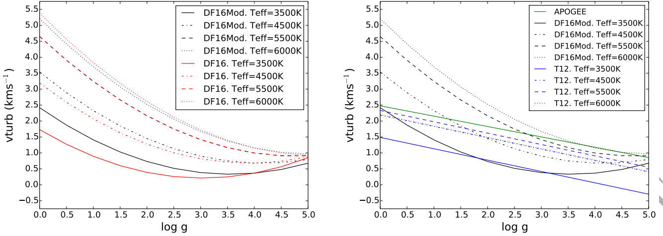
Figure 1. Left Panel: Microturbulent velocity as a function of \log g for the original Dutra-Ferreira et al. 2016 equation (DF16 Red lines) and the modified version of the equation (DF16Mod black lines) for four values of T_{\text{eff}} . For T_{\text{eff}}=5500\text{K} , DF16=DF16Mod. The main difference can be seen at lower temperatures, where DF16Mod avoids dropping to such low values of microturbulent velocity. This modification better represents the trends found by observations (e.g. Ramírez et al. 2013 , their figure 5). Right Panel: Microturbulent velocity as a function of \log g for the modified DF16 equation (DF16Mod, Black lines), the Thygesen et al. 2012 equation (T12, Blue lines) and the APOGEE equation (APOGEE, Green lines). Although the T12 equation appears to follow the linear behaviour of the APOGEE calibration well, problems arise at higher T_{\text{eff}} where the equation does not reach the higher values of microturbulent velocity observed at low \log g .
