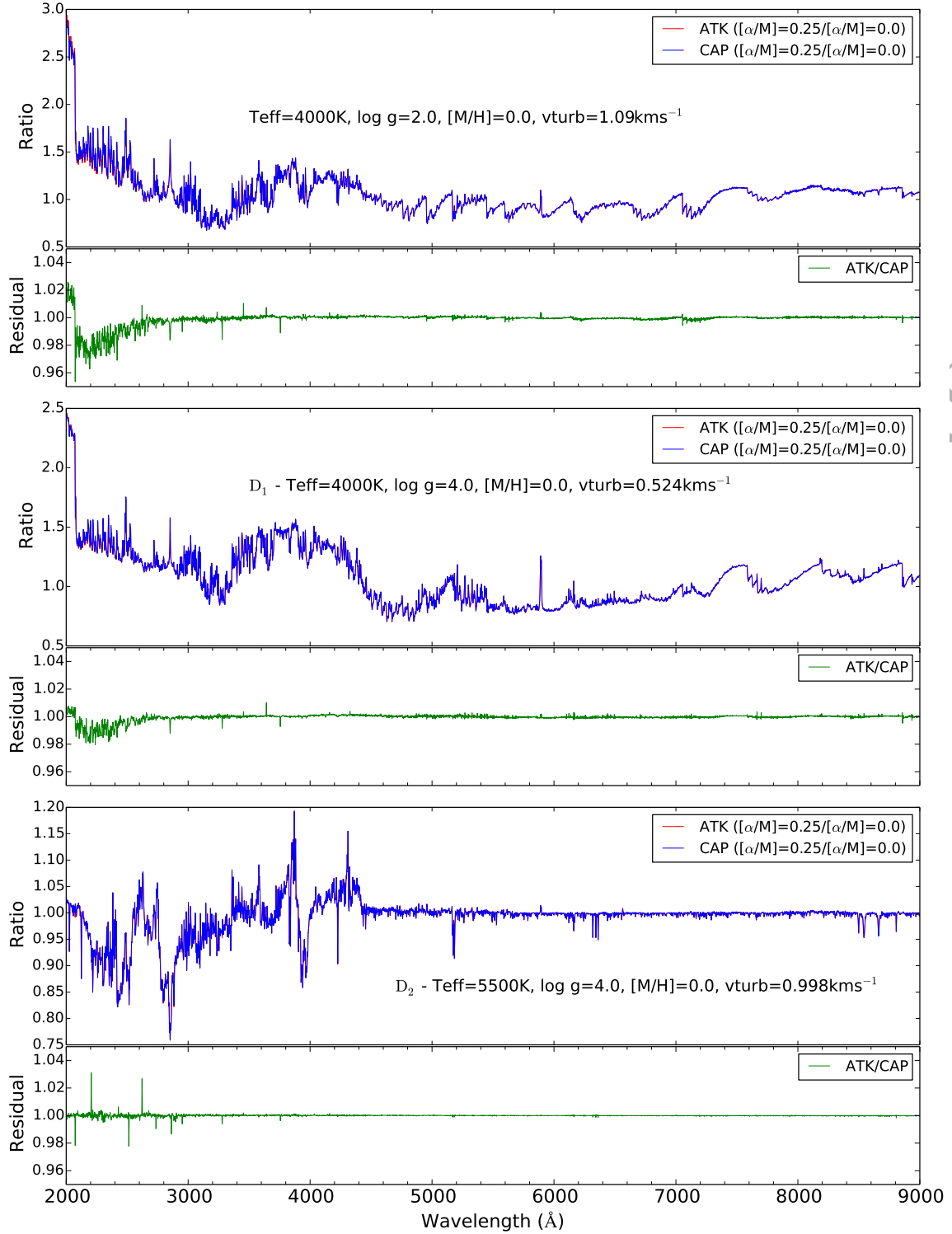
Figure 5. Comparisons of enhanced-over-base star spectra for stars in our theoretical library, labelled ATK, versus stars from Allende Prieto et al. 2018 (interpolated in v_{\text{turb}} ), labelled CAP. The top plot in each block shows spectra for [\alpha/M]=+0.25 divided by [\alpha/M]=0.0 . The lower plot in each block shows the division of these two ratios (ATK/CAP). Blocks show comparisons for a giant star (upper) and two dwarf stars (middle and lower), all at solar metallicity, with parameters detailed in Table 1.
