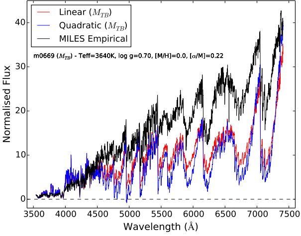
Figure A2. Comparison between the resulting spectra of a linear and quadratic Bézier interpolation, near grid edges, compared to the corresponding empirical spectrum. Spectra are normalised to the flux at 3540.5 Å. The quadratic interpolation produces negative fluxes between \sim 4810 - 4974 Å. A linear interpolation fixes this problem and produces a closer match to the corresponding empirical spectrum for m0669 (HD167006, black line).
