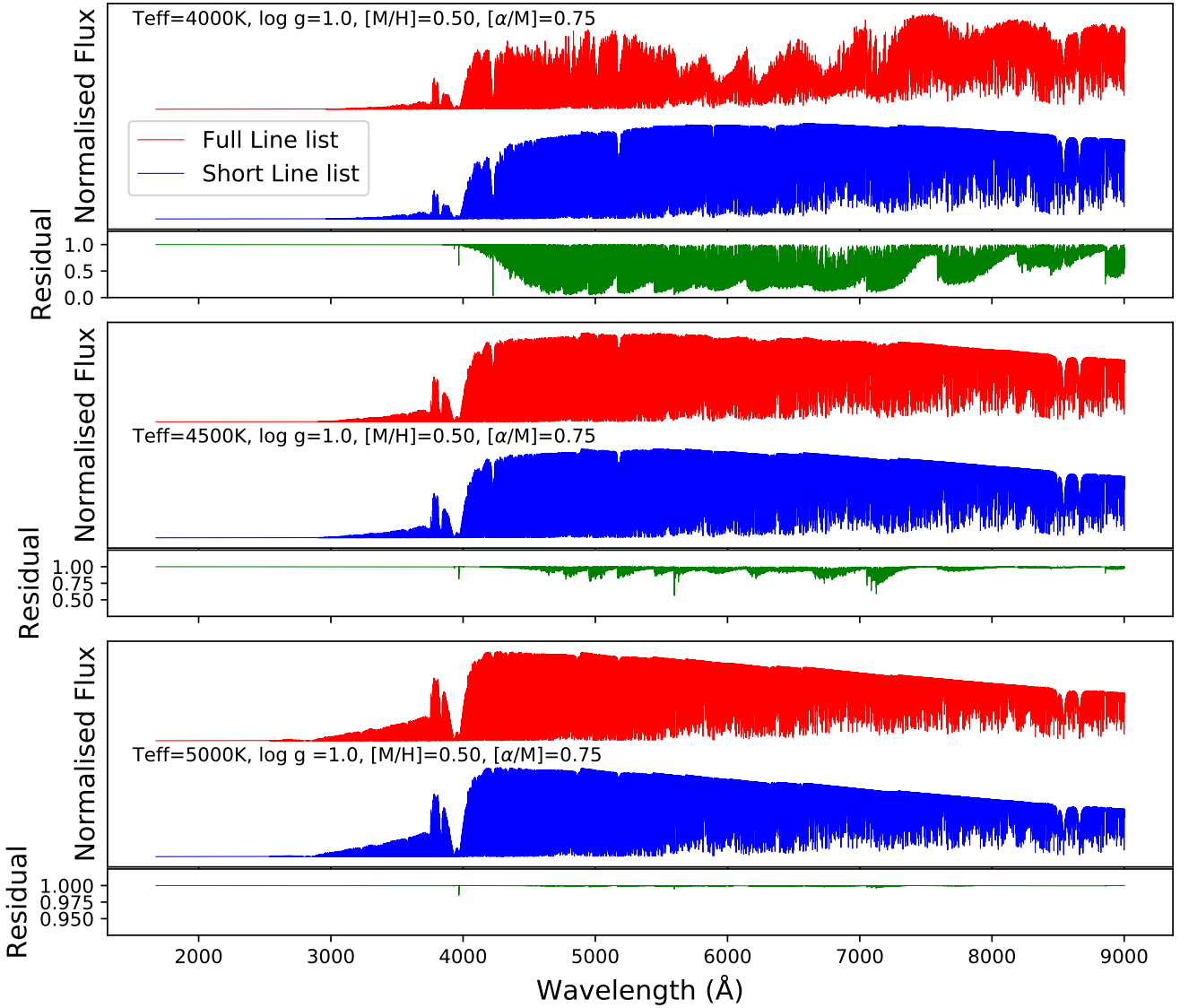
Figure 4. Effect of removing TiO lines from molecular line list at different temperatures for the fixed binning, high-resolution library described in Section 2.6
