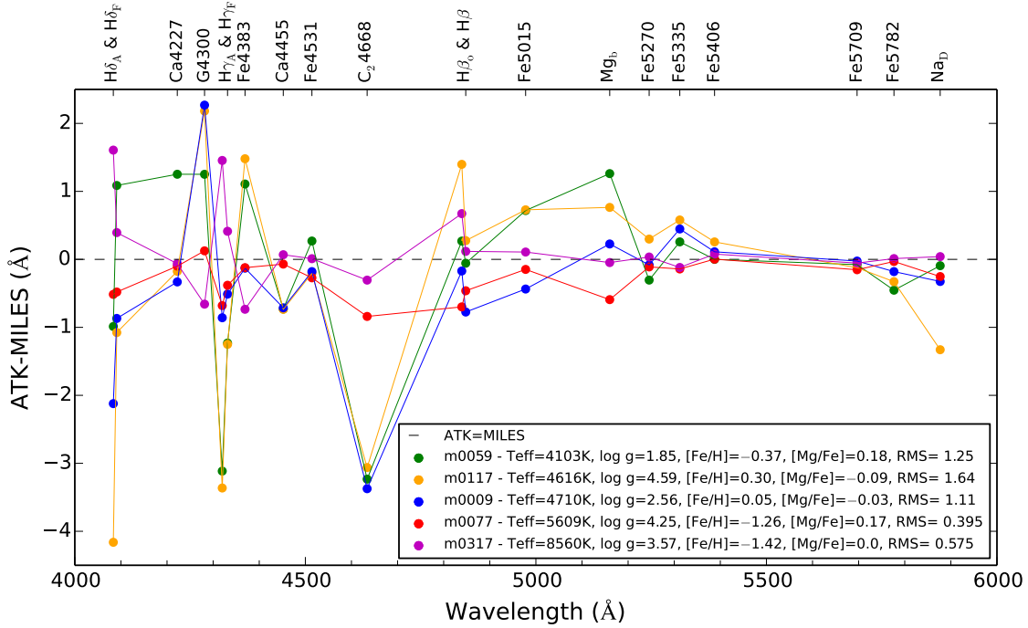
Figure 14. Comparison of Lick indices predicted by our interpolated MILES models (labeled ATK) to empirical MILES stars. This is for indices that are measured in Å, including H\beta_0 from Cervantes & Vazdekis (2009) and for five examples of stars present in the MILES library. Lick indices are labelled for illustration and the 1:1 agreement between model and observation is plotted as a dashed horizontal line. Disagreements between models and observations are generally larger in the blue. RMS scatter (in Å) about the 1:1 agreement line is given for each star.
