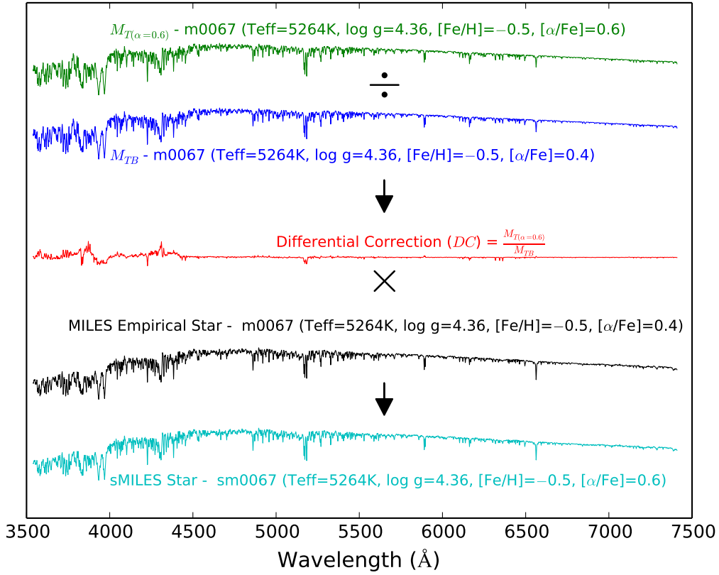
Figure 9. The differential correction method followed for computing \alpha -enhanced and \alpha -deficient semi empirical (sMILES) star spectra. MILES star m0067 is shown as an example. Fully theoretical \alpha -enhanced ( [\alpha/\text{Fe}] = +0.6 ; shown in green) and base (shown in blue) star spectra, are divided to obtain a differential correction (in red). This correction is applied to the corresponding empirical MILES star spectrum (shown in black). The result is a semi-empirical MILES star spectrum (shown in cyan) with a different [\alpha/\text{Fe}] ratio from the original empirical star.
