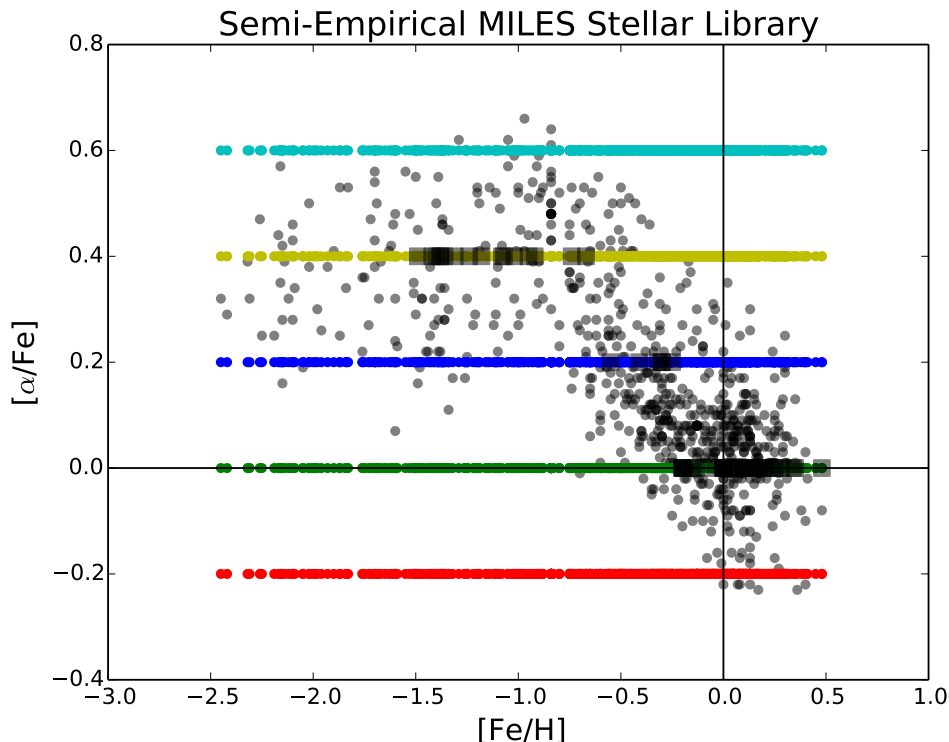
Figure 12. Final semi-empirical MILES (sMILES) stellar library coverage in the [\alpha/\text{Fe}] vs [\text{Fe}/\text{H}] plane. The coloured points that lie in horizontal lines represent the families of 801 sMILES stars and black points represent the corresponding 801 empirical MILES stars, with black squares representing those stars with [\text{Mg}/\text{Fe}] values estimated from a Milky Way relation derived in Bensby et al. (2014) and black circles representing the 752 MILES stars for which Milone et al. (2011) provides [\text{Mg}/\text{Fe}] values.
