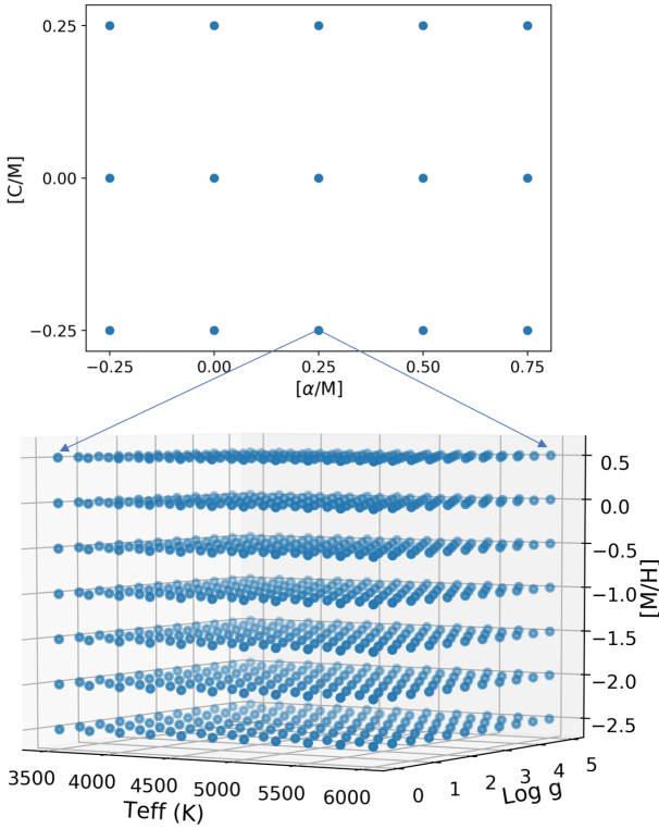
Figure 3. Top Panel: Abundance pattern coverage in the [C/M] vs [\alpha/M] plane. Bottom Panel: 3D stellar parameter coverage of 3500-6000K grid. Each point in the [C/M] vs [\alpha/M] plane represents 11 \times 11 \times 7 = 847 models in this lowest T_{\text{eff}} grid.
