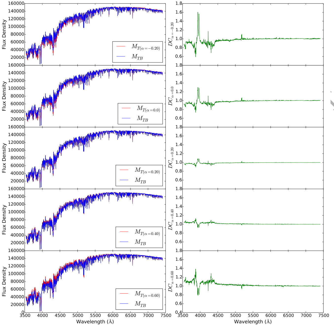
Figure 11. Example of Differential corrections, which are applicable for MILES star m0923 in the globular cluster M3 (=M3 IV 25: T_{\text{eff}}=4367\text{K} , \log g=1.27 , [\text{Fe}/\text{H}]=-1.34 , [\text{Mg}/\text{Fe}]=0.30 ). This empirical MILES star has a [\text{Mg}/\text{Fe}] value of 0.3. The left panel compares the resulting spectra of the theoretical enhanced (or deficient) ( M_{T(\alpha=x)} ) and theoretical base M_{TB} stars. In these plots ( \alpha=x ) is short for ( [\alpha/\text{Fe}]=x ). Flux Density is in units of \text{erg/s/cm}^2/\text{\AA} . The right panel shows the resulting differential correction ( DC_{(\alpha=x)} ), derived from equation (7), for each of the output [\alpha/\text{Fe}] abundances.
