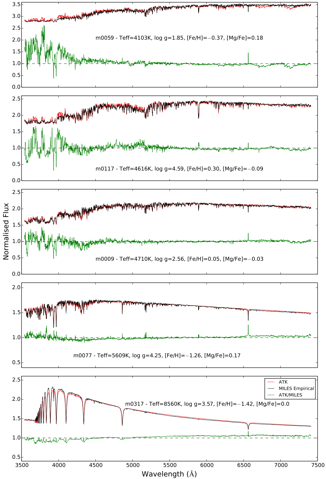
Figure 13. Comparison of ATK model and empirical MILES stars for m0009, m0059, m0077, m00117, m0317. MILES star parameters from Cenarro et al. (2007) and Milone et al. (2011) are given in each panel. Spectra are degraded to 2.5 Å, sampled at 0.9 Å and normalised to unity area. ATK (red lines) and MILES (black lines) spectra are scaled up by a factor of 2000 and shifted onto the plots. Ratios between ATK models and MILES stars are given in the lower panel of each plot (green lines) with no scaling or shifting applied. The vertical axes on the plots are to scale for the ratios between ATK models and MILES stars. The 1:1 agreement between ATK models and MILES empirical star is represented as a dashed-horizontal line.
