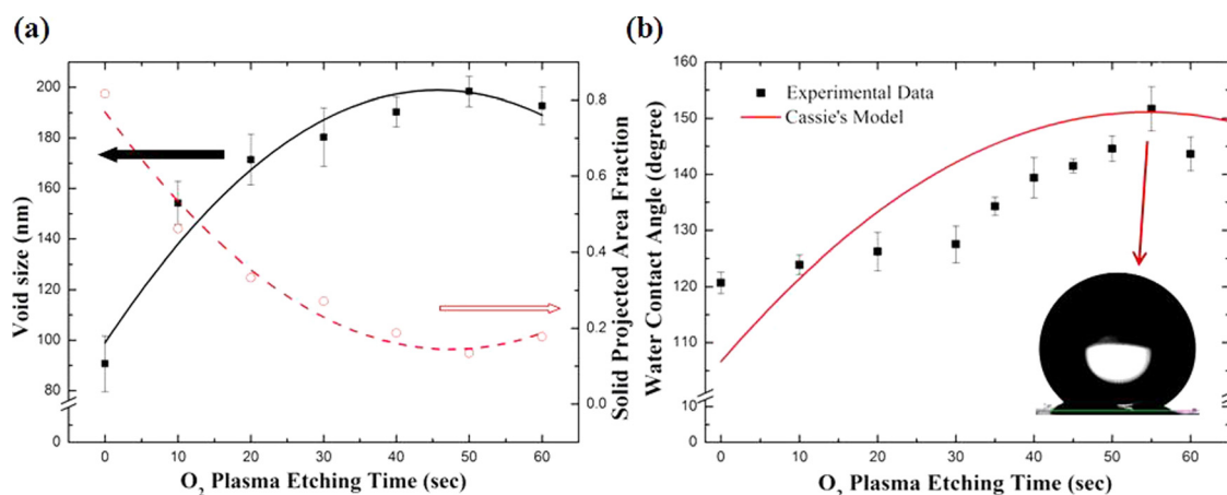
FIG. 4. (a) Dependence of the void size and the corresponding projected area fraction of macroporous ETPTA films template from 200 nm silica microspheres at different oxygen plasma etching durations. (b) Experimental and calculated static water contact angles of the surface modified macroporous films etched at different oxygen plasma etching durations.
