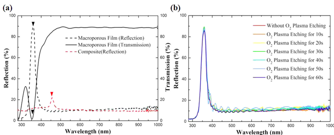
FIG. 5. (a) Normal incidence optical spectra of a silica colloidal crystal-ETPTA composite consisting of 200 nm silica microspheres, and a corresponding macroporous ETPTA film. The arrows indicate the expected positions of the peaks for each sample, calculated using Bragg's law at normal incidence. (b) Normal incidence optical reflection spectra obtained from macroporous ETPTA films fabricated by oxygen plasma etching a composite at different durations.
